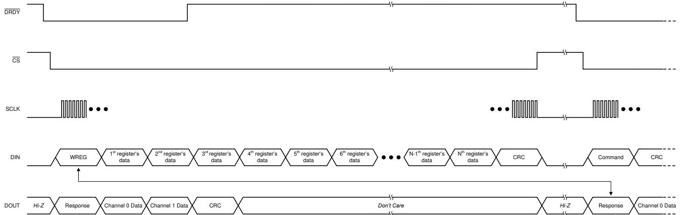
Figure 8-25. Writing Registers
