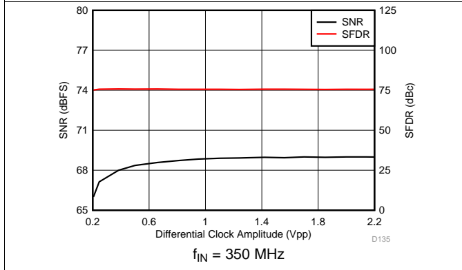
Figure 37. Performance vs Differential Clock Amplitude
