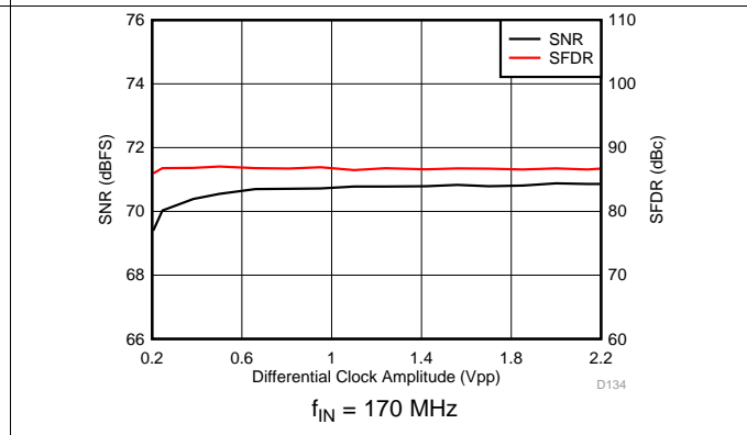
Figure 36. Performance vs Differential Clock Amplitude
