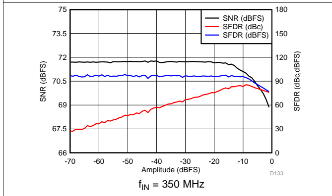
Figure 35. Performance vs Amplitude
