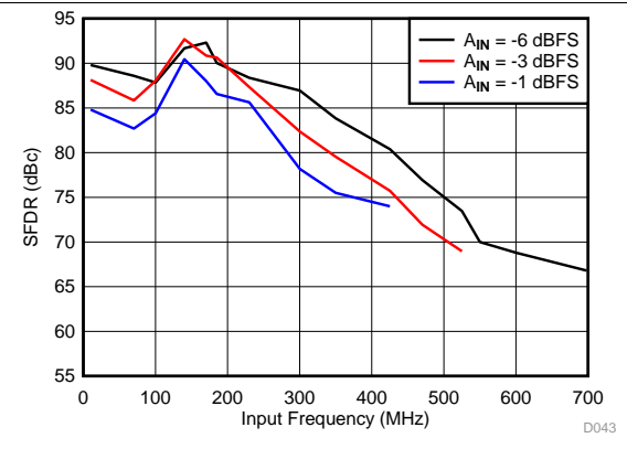
Figure 20. Spurious-Free Dynamic Range vs Input Frequency
