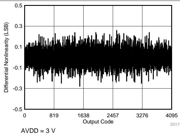
⊠ 17. Typical DNL in Manual Mode
