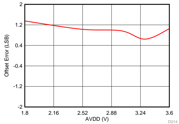
⊠ 14. Offset Error in Manual Mode with AVDD
