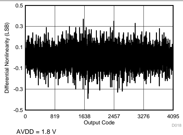
⊠ 18. Typical DNL in Manual Mode
