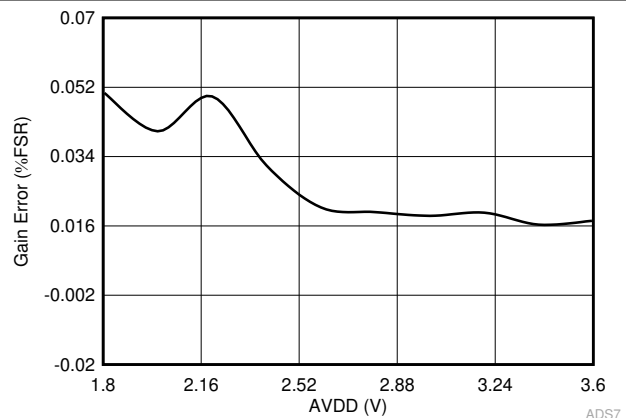
6-16. Gain Error in Manual Mode vs AVDD
