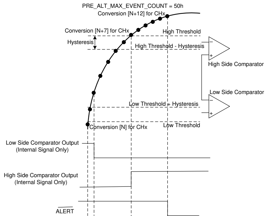
8-5. Out of Range Alert With the ADS7142-Q1
