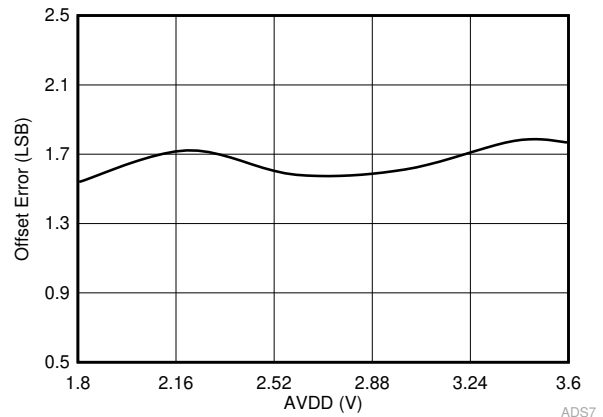
6-14. Offset Error in Manual Mode vs AVDD
