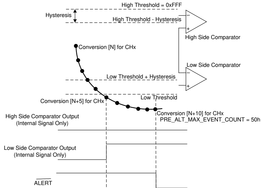
8-3. Low Alert With the ADS7142-Q1
