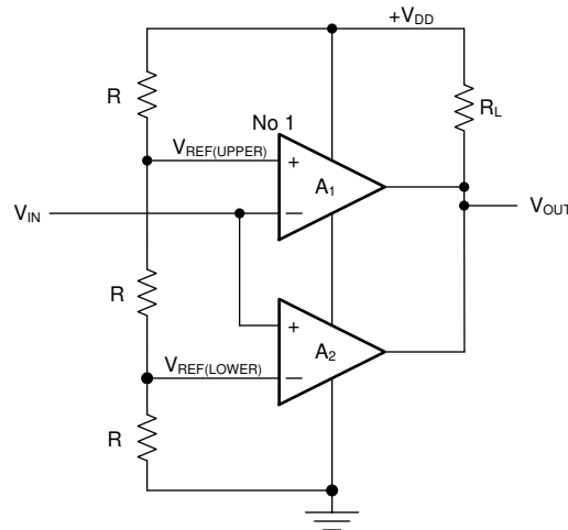
図 8-1. Analog Window Comparator
