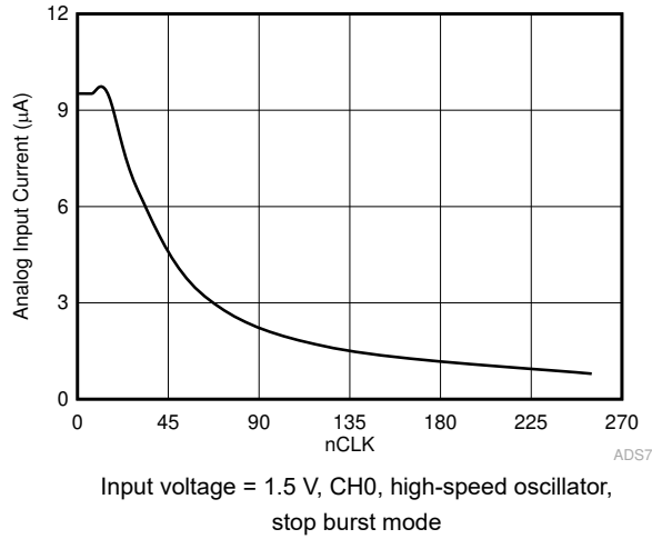
6-29. Analog Input Current in Autonomous Modes vs nCLK
