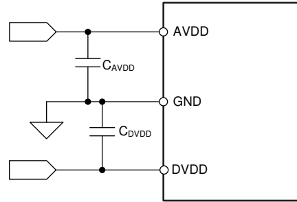
8-9. Power-Supply Decoupling
