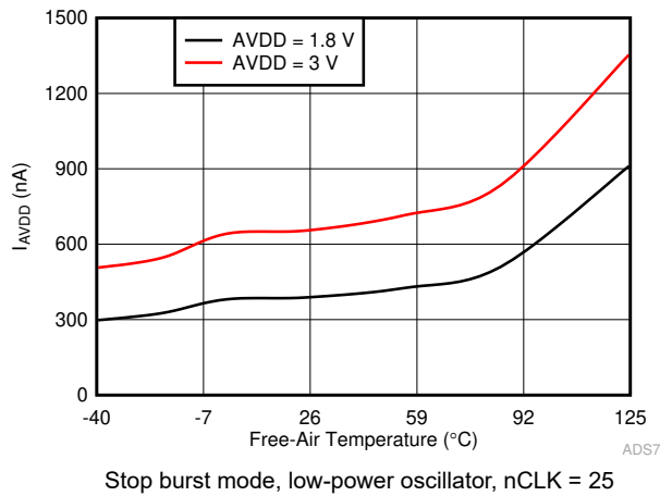
6-31. I_{AVDD} in Autonomous Modes vs Temperature
