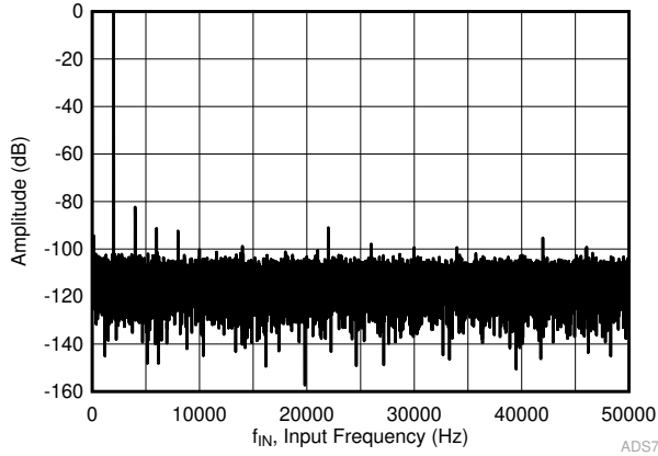
6-5. Typical FFT in Manual Mode
