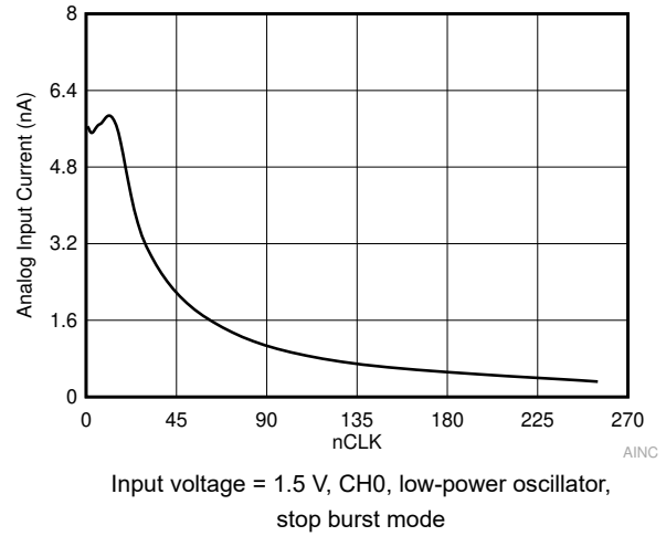
6-30. Analog Input Current in Autonomous Modes vs nCLK
