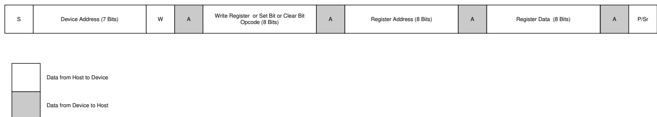
7-29. Writing a Single Register
