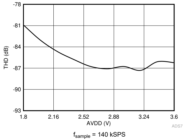
6-11. THD in Manual Mode vs AVDD
