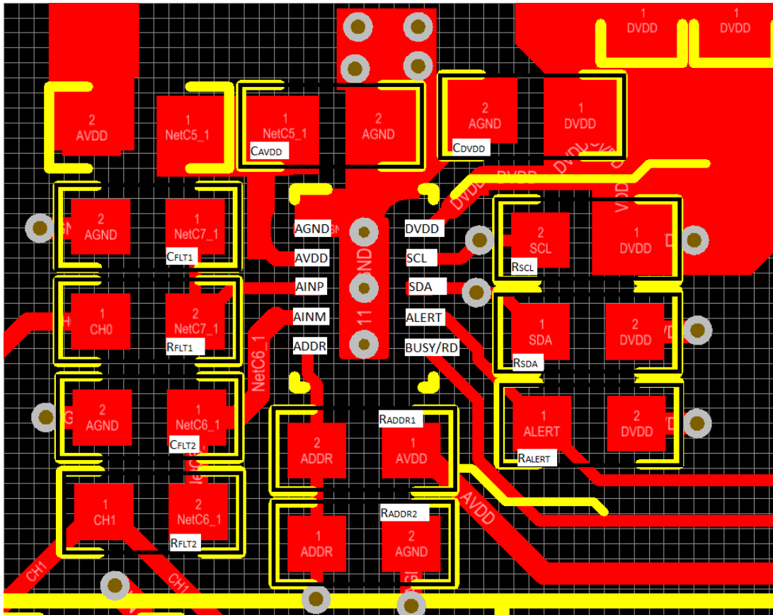
8-11. Example Layout
