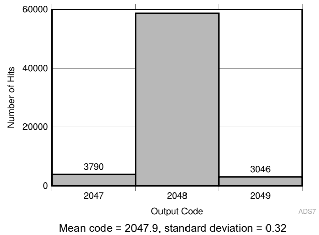
6-12. Typical DC Code Spread in Manual Mode
