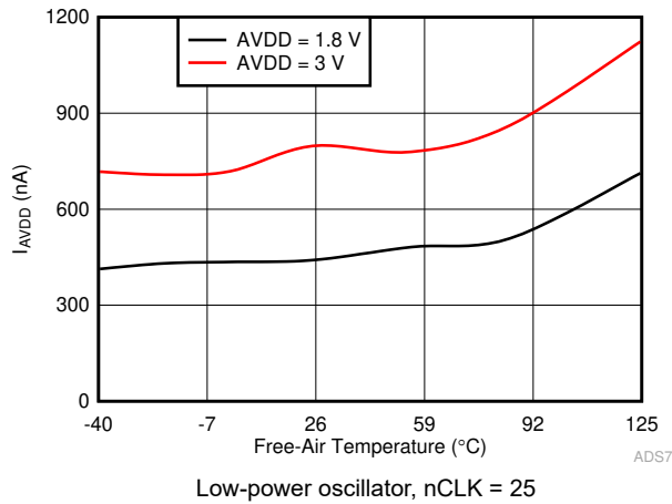
6-35. I_{AVDD} in High-Precision Mode vs Temperature Low-power oscillator, nCLK = 25
