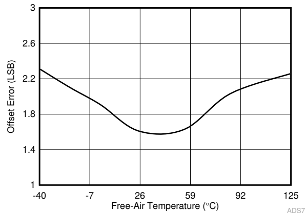
6-13. Offset Error in Manual Mode vs Temperature
