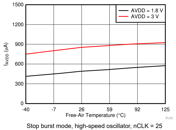
6-32. I_{AVDD} in Autonomous Modes vs Temperature
