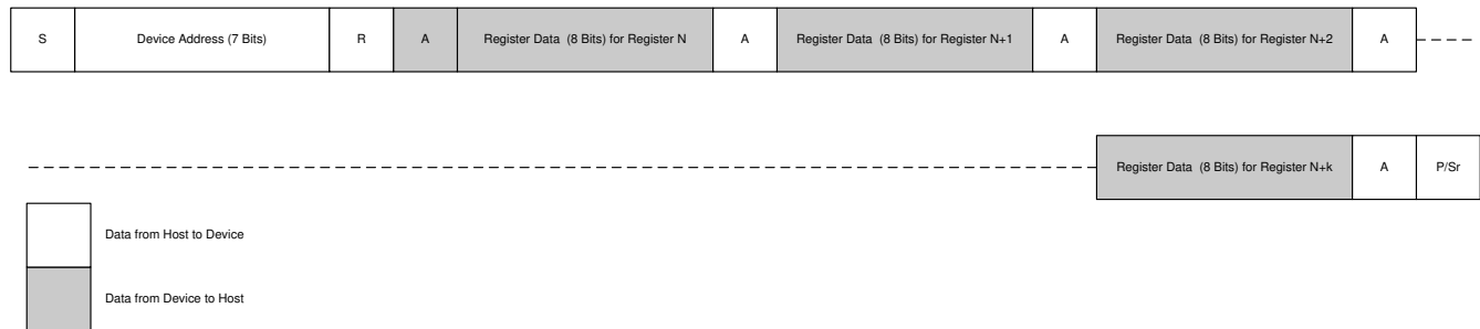
7-28. Reading a Continuous Block of Registers
