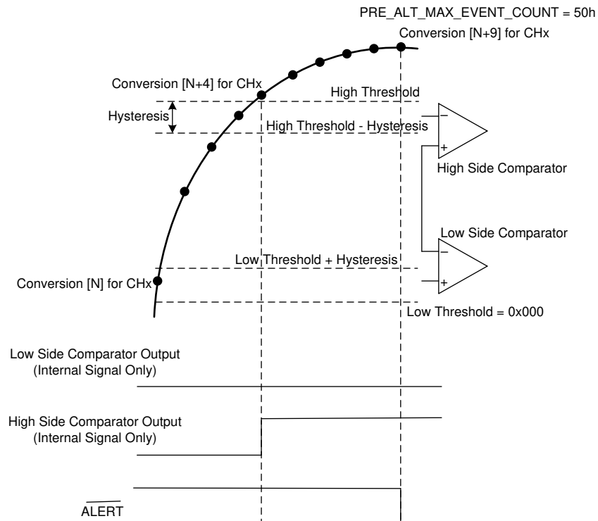
8-4. High Alert With the ADS7142-Q1
