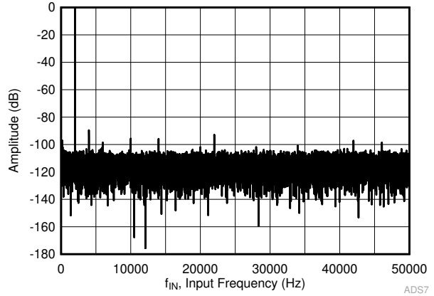
6-6. Typical FFT in Manual Mode
