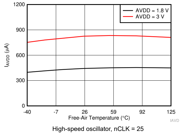
6-36. I_{AVDD} in High-Precision Mode vs Temperature High-speed oscillator, nCLK = 25
