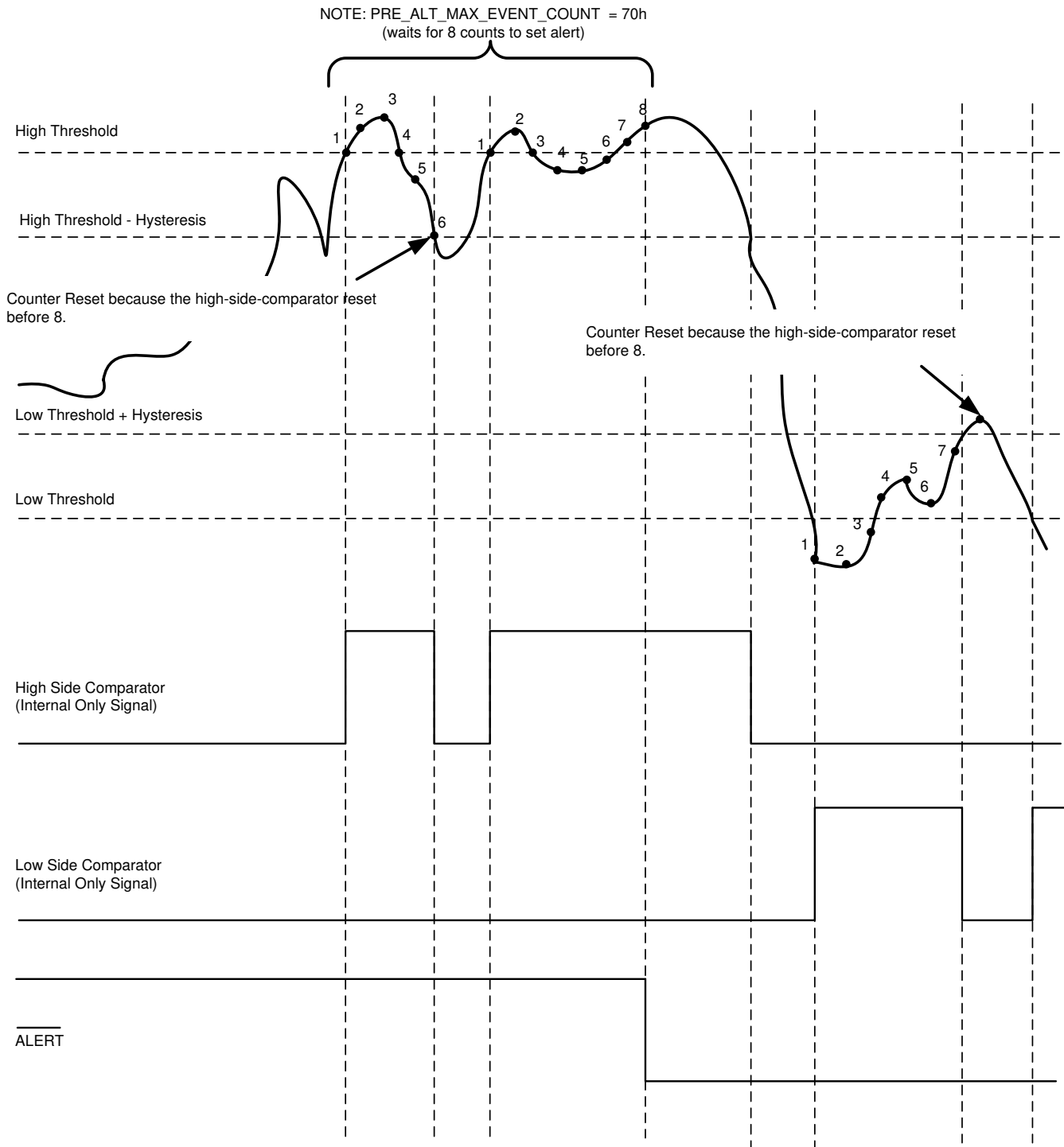
7-10. Thresholds, Hysteresis, and Event Counter for the Digital Window Comparator
