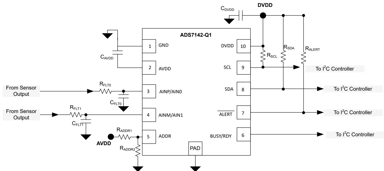
8-10. Example Schematic
