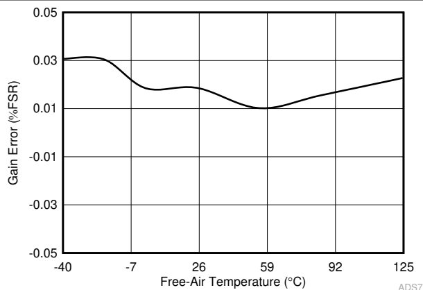
6-15. Gain Error in Manual Mode vs Free-Air Temperature
