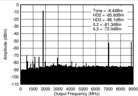
5-345. TX Single Tone (-1 dBFS) Output Spectrum at 1.8 GHz ( 0-f_{\text{DAC}} )
