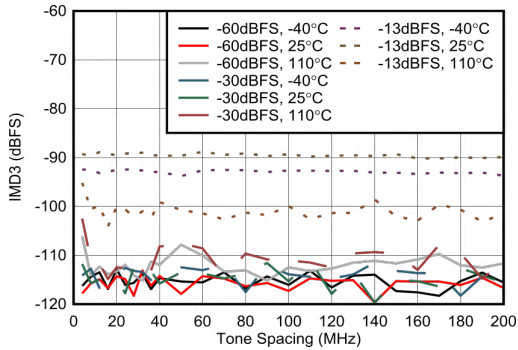
5-123. RX IMD3 vs Tone Spacing at 2.6 GHz (Ext. Clock)
