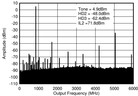
5-328. TX Single Tone (-6 dBFS) Output Spectrum at 0.85 GHz ( 0-f_{\text{DAC}} )
