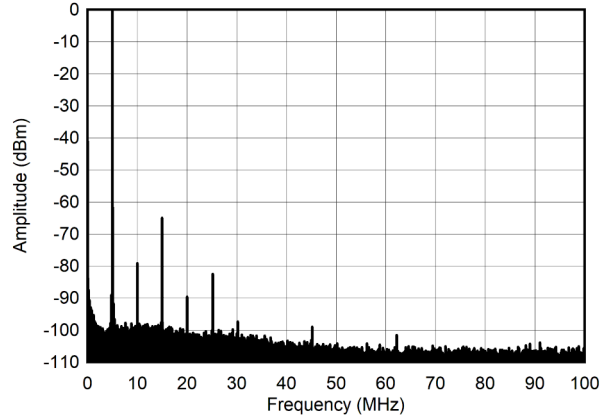
5-215. Single Tone Spectrum at 5 MHz and -6 dBFS (0 - 100 MHz)
