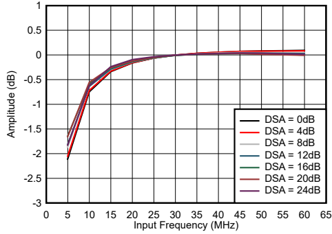
5-1. RX In-Band Gain Flatness, f_{IN} = 30\text{ MHz}
