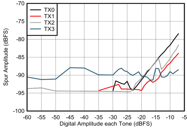
5-393. Two Tone Inband SFDR vs Digital Amplitude at 2.6 GHz
