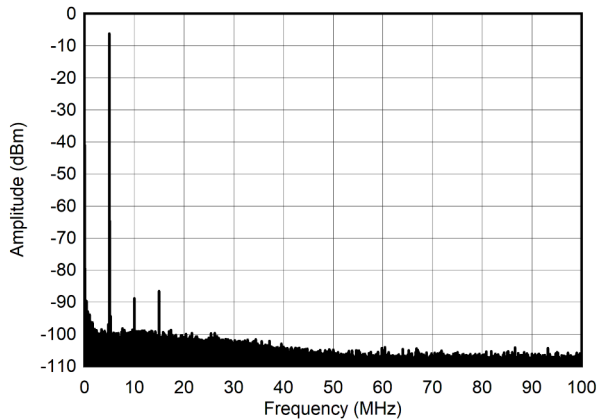
5-216. Single Tone Spectrum at 5 MHz and -12 dBFS (0 - 100 MHz)
