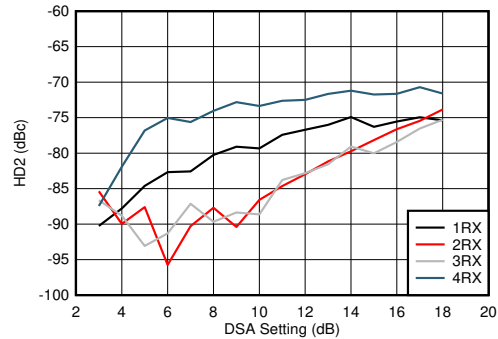
5-124. RX HD2 vs DSA Setting and Channel at 2.6 GHz
