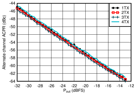
5-505. TX 20-MHz LTE ACPR vs Digital Level at 4.9 GHz
