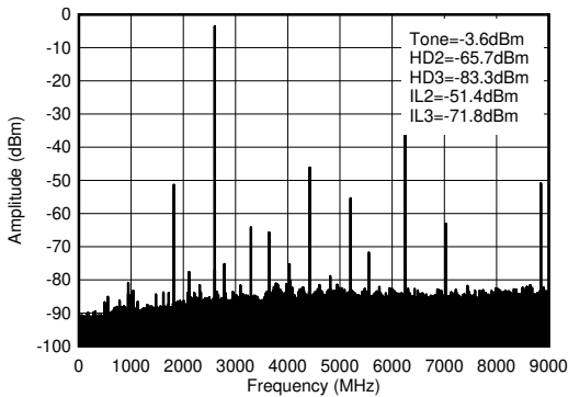
5-395. TX Single Tone (-12 dBFS) Output Spectrum at 2.6 GHz ( 0-f_{\text{DAC}} )
