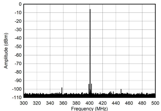
5-253. Single Tone Spectrum at 400 MHz and -12 dBFS ( \pm 100 MHz)
