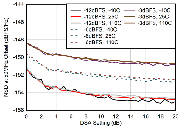
5-44. NSD vs DSA Setting at 400MHz
