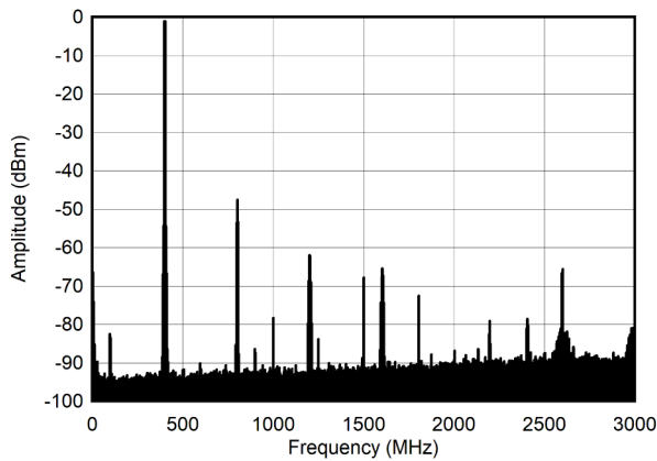
5-258. Dual Tone Spectrum at 400 MHz and -7 dBFS (Nyquist)
