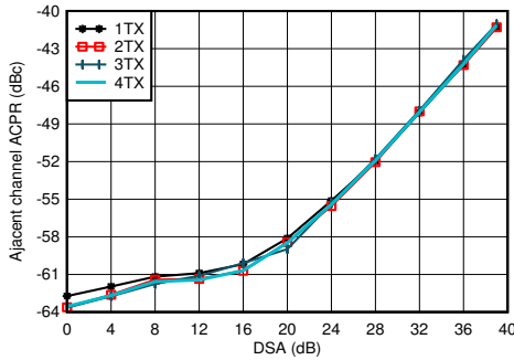
3.5 GHz Matching, single carrier 100-MHz BW NR TM1.1 5-454. TX 100-MHz NR ACPR vs DSA Setting at 3.5 GHz
