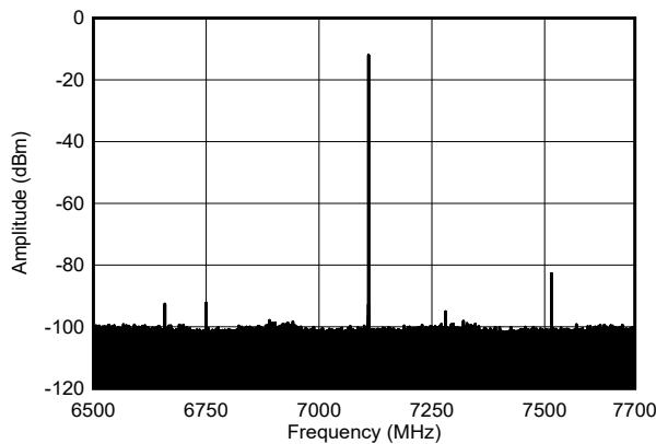
5-556. Single Tone Output Spectrum at 7.1GHz, -1dBFS (Inband)
