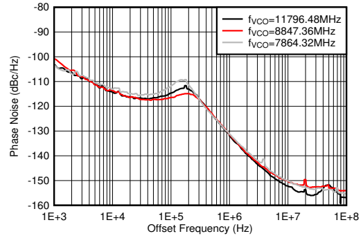
5-569. Phase Noise vs Offset Frequency and f_{VCO} at f_{OUT} = 2610\text{ MHz}
