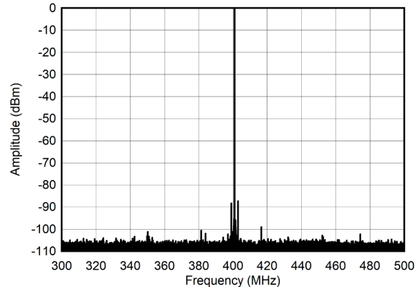
5-251. Single Tone Spectrum at 400 MHz and -6 dBFS ( \pm 100 MHz)
