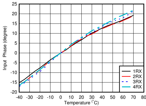
5-83. RX Input Phase vs Temperature and DSA at f_{IN} = 1.75\text{ GHz}
