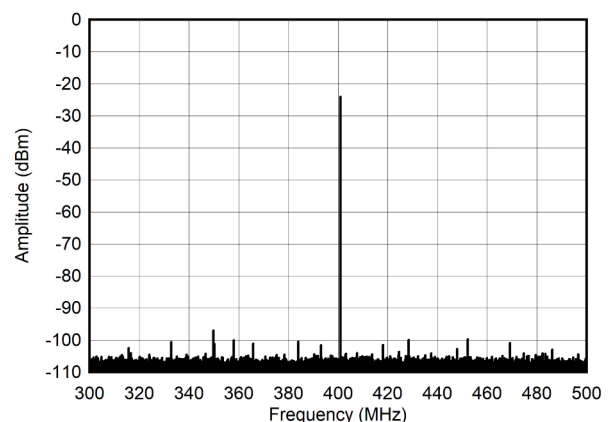
5-255. Single Tone Spectrum at 400 MHz and -30 dBFS ( \pm 100 MHz)
