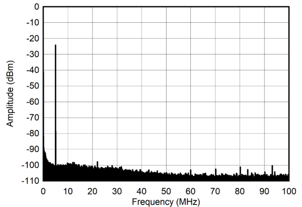
5-217. Single Tone Spectrum at 5 MHz and -30 dBFS (0 - 100 MHz)
