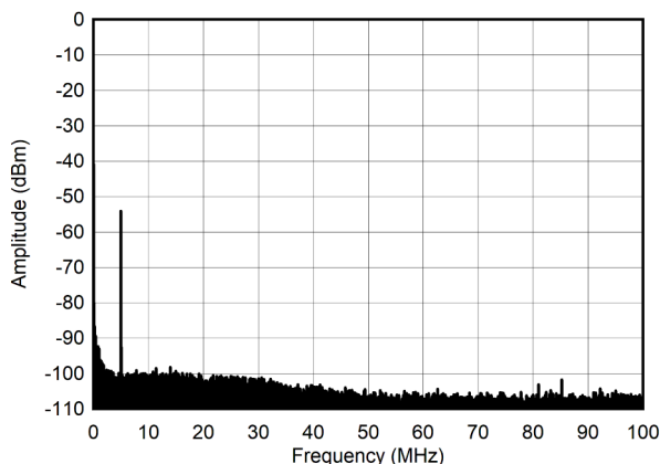
5-218. Single Tone Spectrum at 5 MHz and -60 dBFS (0 - 100 MHz)
