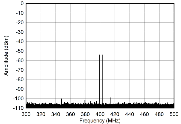
5-265. Dual Tone Spectrum at 400 MHz and -60 dBFS (±100MHz)
