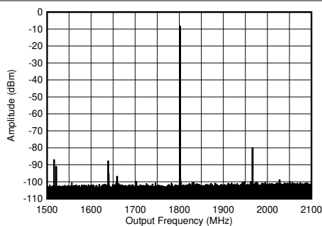
5-346. TX Single Tone (-1 dBFS) Output Spectrum at 1.8 GHz ( \pm 300\text{ MHz} )
