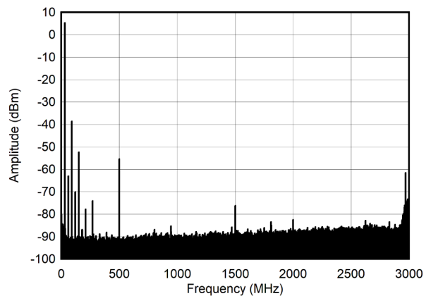
5-219. Single Tone Spectrum at 30 MHz and -1 dBFS (Nyquist)
