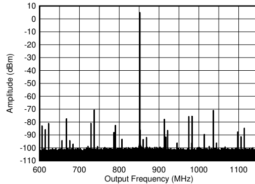
5-329. TX Single Tone (-6 dBFS) Output Spectrum at 0.85 GHz ( \pm 300\text{ MHz} )
