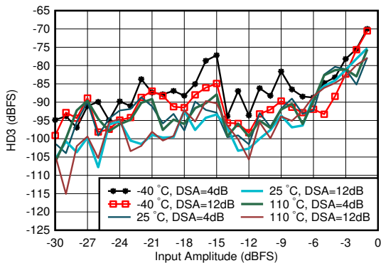
5-74. RX HD3 vs DSA Setting and Temperature at 0.8 GHz
