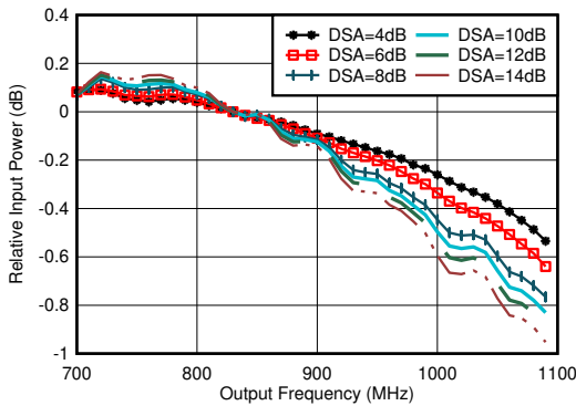
5-50. RX In-Band Gain Flatness for Channel 1RX, f_{IN} = 830 MHz
