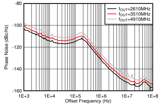
5-571. Phase Noise for 12-GHz VCO vs Offset Frequency and f_{OUT} at 25^\circ\text{C}
