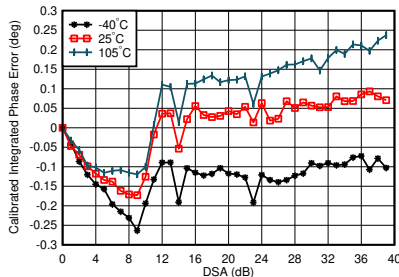
5-371. TX Calibrated Differential Phase Error vs DSA Setting and Temperature at 2.6 GHz
