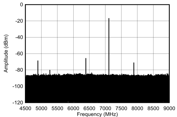
5-557. Single Tone Output Spectrum at 7.1GHz, -6dBFS (Nyquist)
