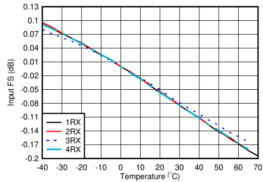
5-51. RX Input Fullscale vs Temperature and Channel at 800MHz
