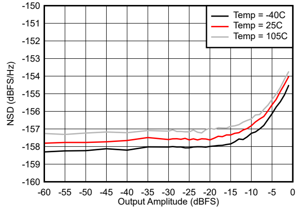
5-233. Noise Spectral Density vs Digital Amplitude at 30 MHz
