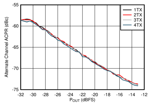
3.5 GHz Matching, single carrier 20-MHz BW TM1.1 LTE 5-457. TX 20-MHz LTE alt-ACPR vs Digital Level at 3.5 GHz
