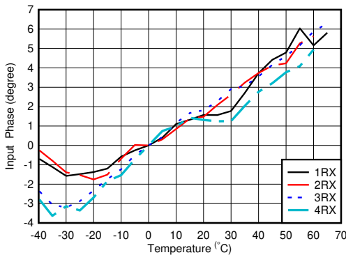
5-52. RX Input Phase vs Temperature and DSA at f_{OUT} = 0.8 GHz
