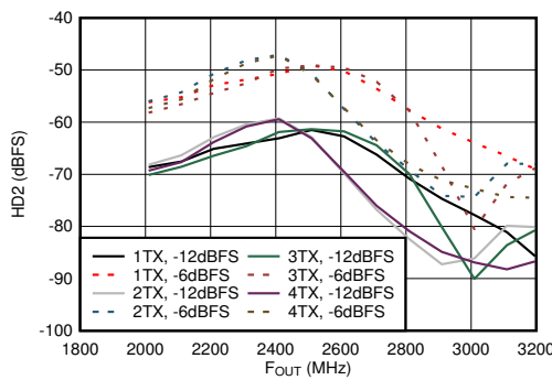
Matching at 2.6 GHz, f_{\text{DAC}} = 11.79648\text{GSPS} , interleave mode, normalized to output power at harmonic frequency
