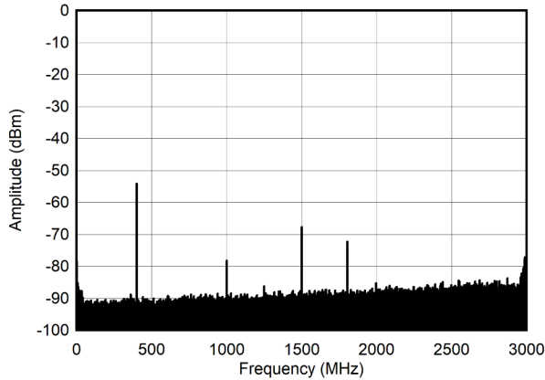
5-256. Single Tone Spectrum at 400 MHz and -60 dBFS (Nyquist)
