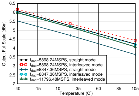
5-278. TX Output Fullscale vs Temperature
