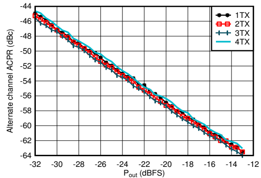
5-506. TX 20-MHz LTE alt-ACPR vs Digital Level at 4.9 GHz
