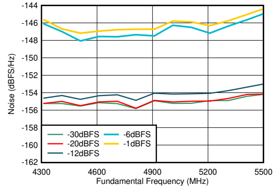
5-498. TX NSD vs Output Frequency and Digital Amplitude at 4.9GHz (DSA=6dB)
