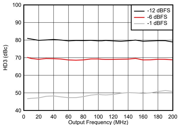
5-237. HD3 vs Frequency 0 - 200 MHz
