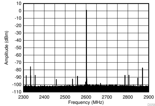
5-406. TX Single Tone (-1 dBFS) Output Spectrum at 2.6 GHz ( \pm 300\text{ MHz} )
