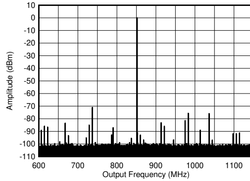
5-329. TX Single Tone (-6 dBFS) Output Spectrum at 0.85 GHz ( \pm 300\text{ MHz} )
