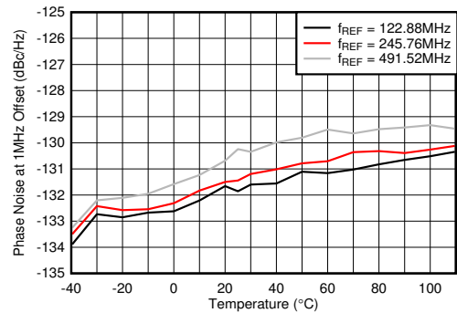
5-589. Phase Noise for 10-GHz VCO at 1 MHz vs Temperature and f_{REF} at f_{OUT} = 2.6 GHz
