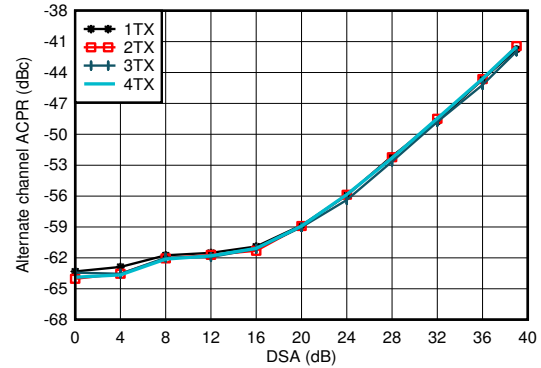
3.5 GHz Matching, single carrier 100-MHz BW NR TM1.1 5-455. TX 100-MHz NR alt-ACPR vs DSA Setting at 3.5 GHz
