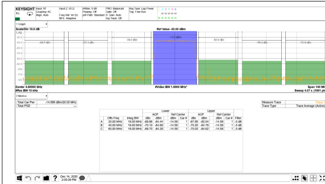
5-503. TX 20-MHz LTE Output Spectrum at 4.9 GHz
