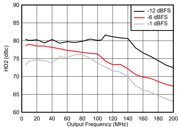
5-236. HD2 vs Frequency 0 - 200 MHz
