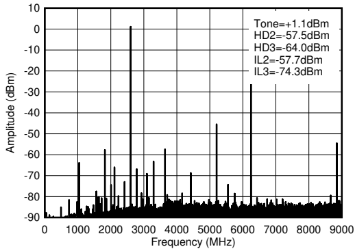
5-403. TX Single Tone (-6 dBFS) Output Spectrum at 2.6 GHz (0- f_{\text{DAC}} )
