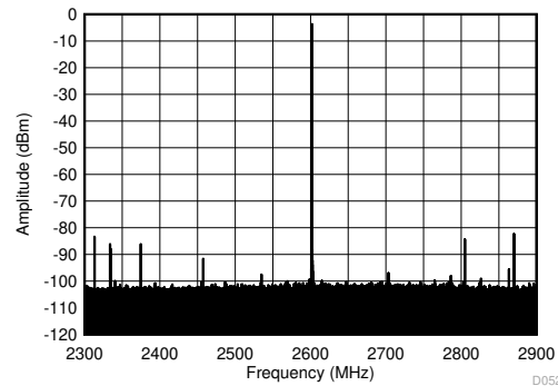
5-396. TX Single Tone (-12 dBFS) Output Spectrum at 2.6 GHz ( \pm 300\text{ MHz} )
