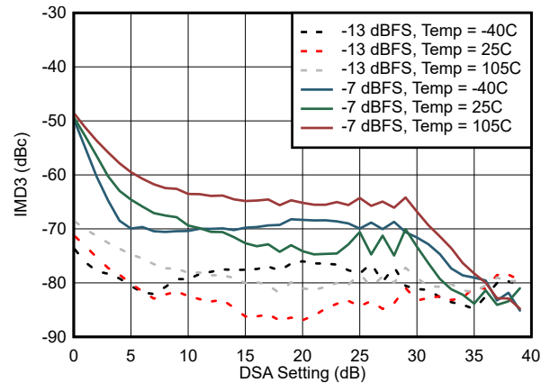
5-235. IMD3 vs DSA Setting at 30 MHz
