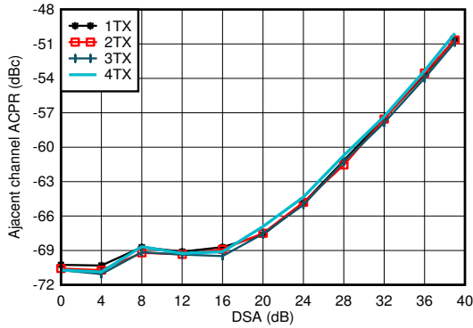
3.5 GHz Matching, single carrier 20-MHz BW TM1.1 LTE 5-452. TX 20-MHz LTE ACPR vs DSA Setting at 3.5 GHz
