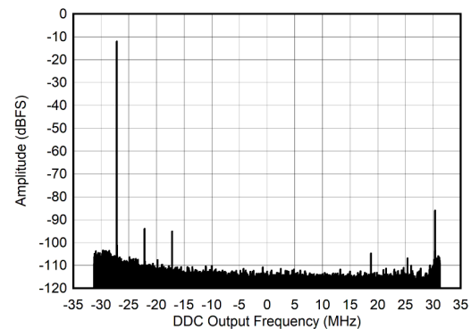
5-12. RX Output FFT at 5 MHz
