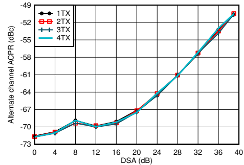
3.5 GHz Matching, single carrier 20-MHz BW TM1.1 LTE 5-453. TX 20-MHz LTE alt-ACPR vs DSA Setting at 3.5 GHz
