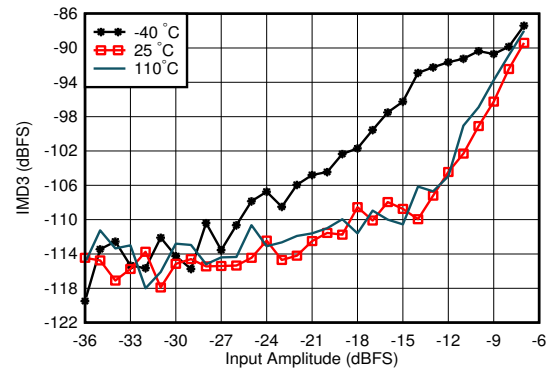
5-67. RX IMD3 vs Input Level and Temperature at 0.8 GHz
