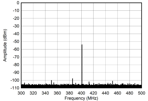
5-257. Single Tone Spectrum at 400 MHz and -60 dBFS ( \pm 100\text{MHz} )
