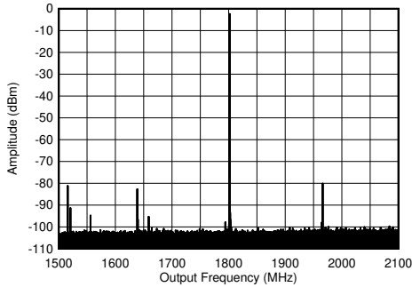
5-350. TX Single Tone (-6 dBFS) Output Spectrum at 1.8 GHz ( \pm 300 MHz)
