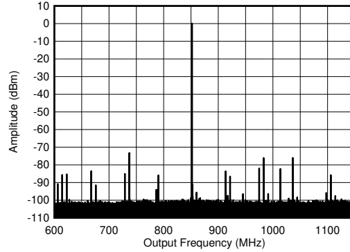
5-323. TX Single Tone (-6 dBFS) Output Spectrum at 0.85 GHz ( \pm 300\text{ MHz} )
