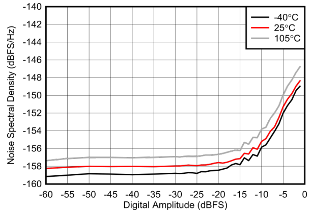
5-420. NSD vs Digital Amplitude and Temperature at 2.6 GHz
