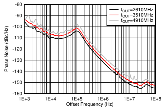
5-571. Phase Noise for 12-GHz VCO vs Offset Frequency and f_{OUT} at 25^\circ\text{C}
