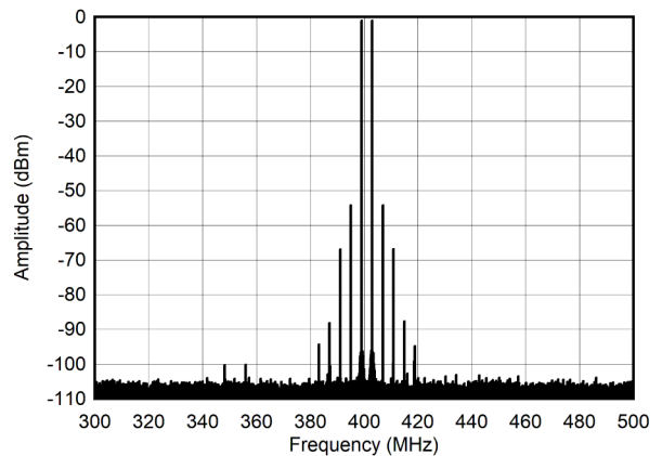
5-259. Dual Tone Spectrum at 400 MHz and -7 dBFS ( \pm 100\text{MHz} )
