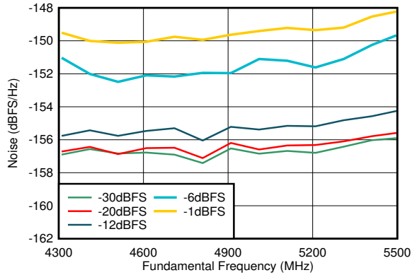
5-497. TX NSD vs Output Frequency and Digital Amplitude at 4.9 GHz (DSA=0dB)
