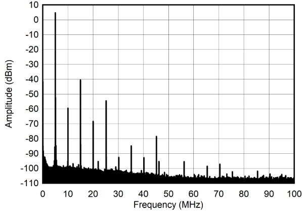
5-214. Single Tone Spectrum at 5 MHz and -1 dBFS (0 - 100 MHz)
