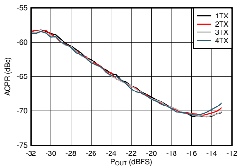
3.5 GHz Matching, single carrier 20-MHz BW TM1.1 LTE 5-456. TX 20-MHz LTE ACPR vs Digital Level at 3.5 GHz
