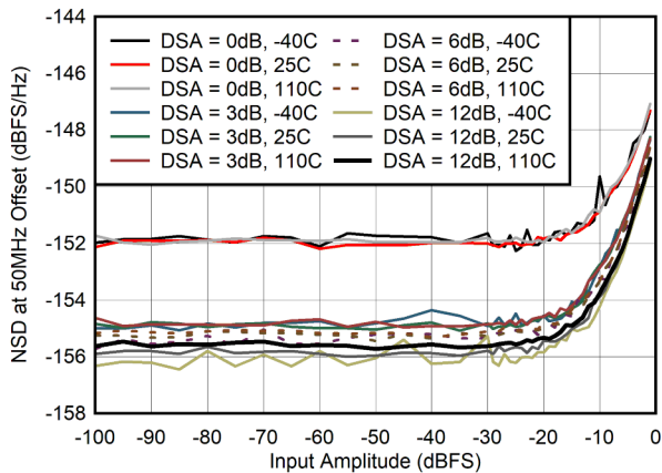
5-43. NSD vs Input Amplitude at 400MHz
