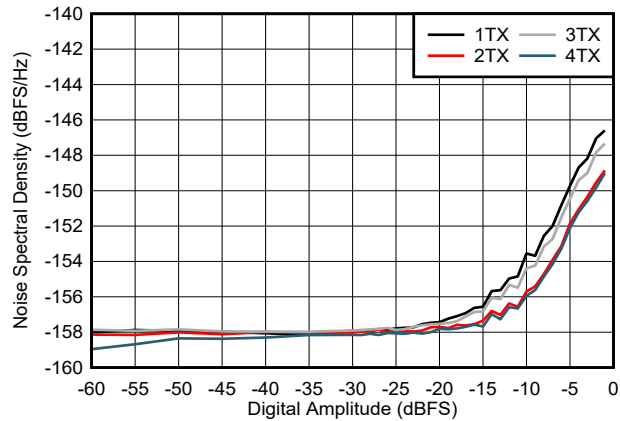
5-419. NSD vs Digital Amplitude and Channel at 2.6 GHz
