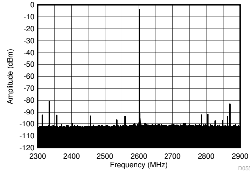
5-404. TX Single Tone (-6 dBFS) Output Spectrum at 2.6 GHz ( \pm 300\text{ MHz} )
