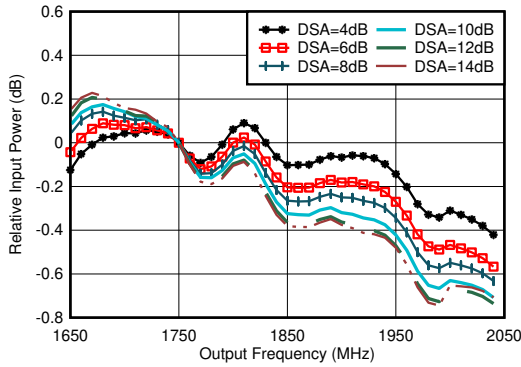
5-81. RX In-Band Gain Flatness, f_{IN} = 1750\text{ MHz}
