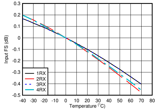
5-82. RX Input Fullscale vs Temperature and Channel at 1.75 GHz
