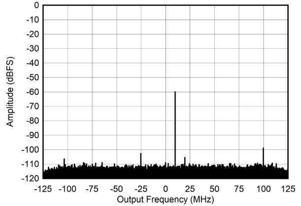
5-42. RX Output FFT at 405 MHz and -60dBFS
