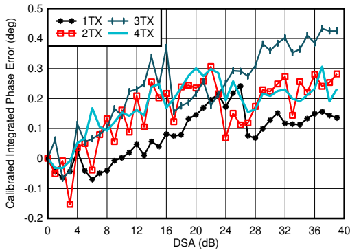
5-489. TX Calibrated Differential Phase Error vs DSA Setting and Channel at 4.9 GHz
