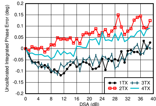
5-366. TX Uncalibrated Differential Phase Error vs DSA Setting and Channel at 2.6 GHz
