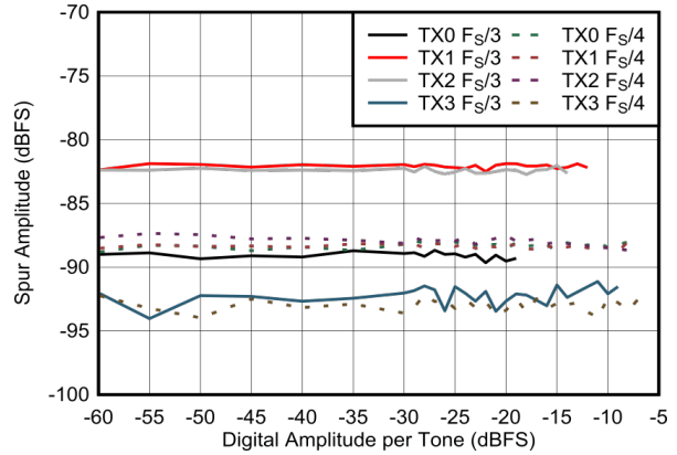
5-394. Two Tone Inband Fixed Spurs vs Digital Amplitude at 2.6 GHz
