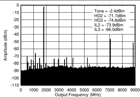
5-347. TX Single Tone (-12 dBFS) Output Spectrum at 1.8 GHz ( 0-f_{\text{DAC}} )
