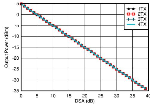
5-279. TX Output Power vs DSA Setting and Channel at 0.85 GHz
