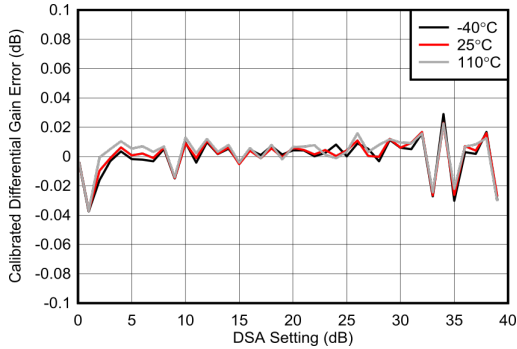
5-528. Calibrated Differential Gain Error vs Temperature at 7.1 GHz
