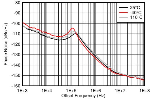
5-598. Phase Noise for 8-GHz VCO vs Offset Frequency and Temperature at f_{OUT} = 1910 MHz
