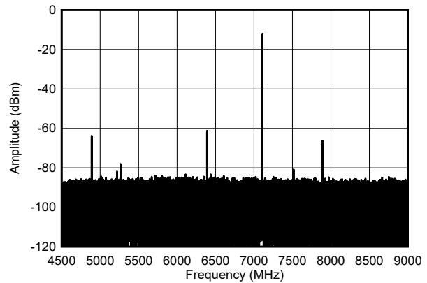
5-555. Single Tone Output Spectrum at 7.1GHz, -1dBFS (Nyquist)
