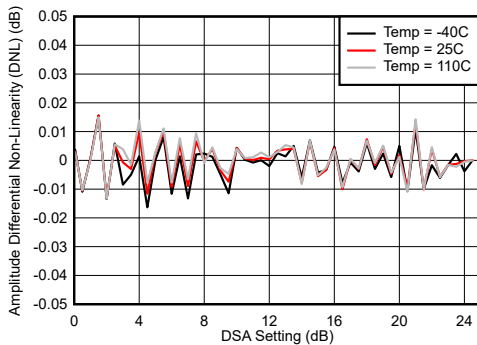
5-3. RX Calibrated Differential Amplitude Error vs DSA Setting at 30 MHz
