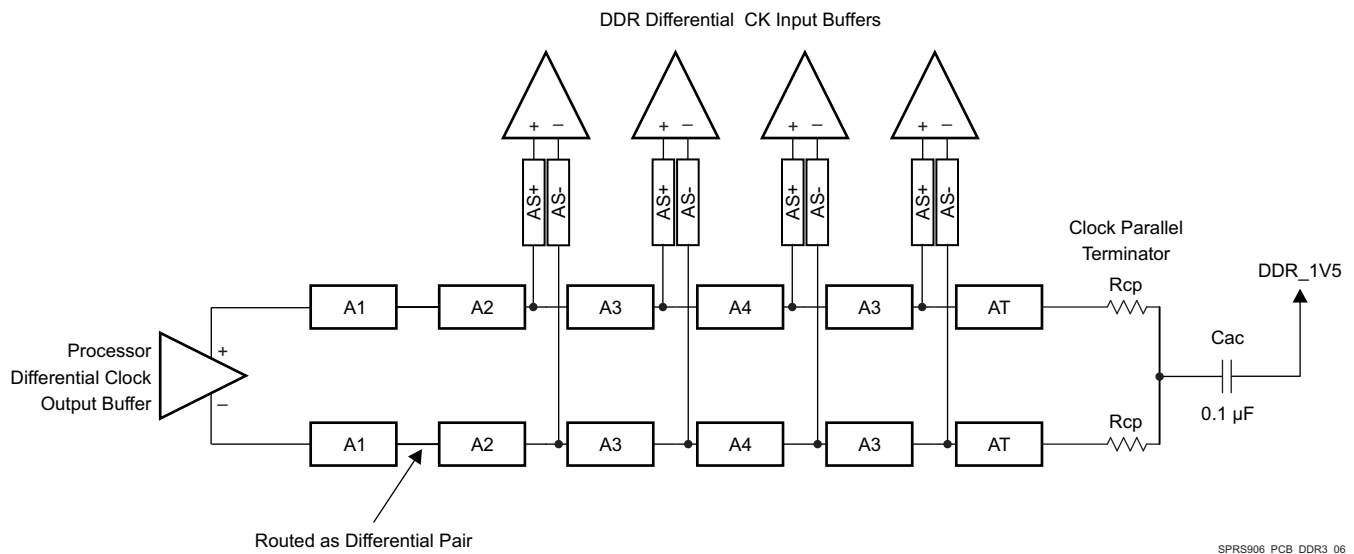
☒ 8-6. CK Topology for Four x8 DDR3 Devices
