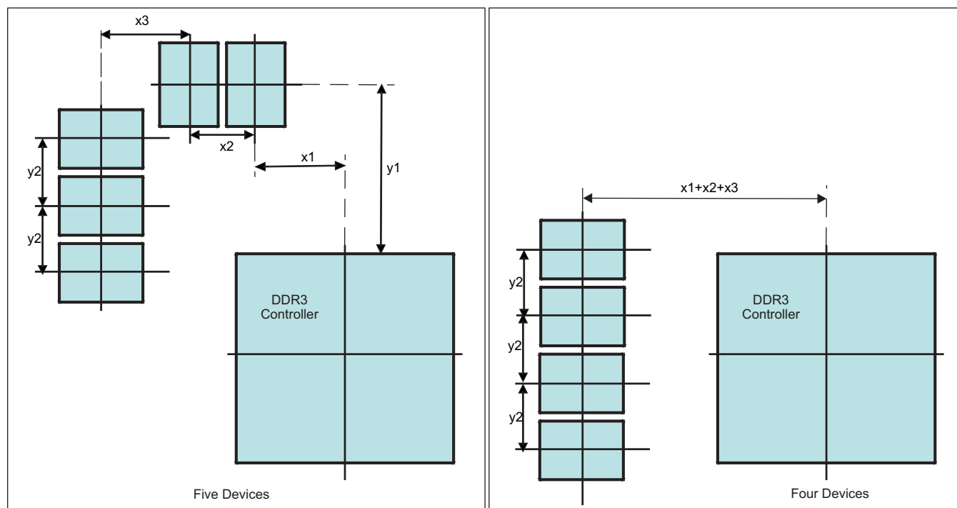
☒ 8-4. Placement Specifications
