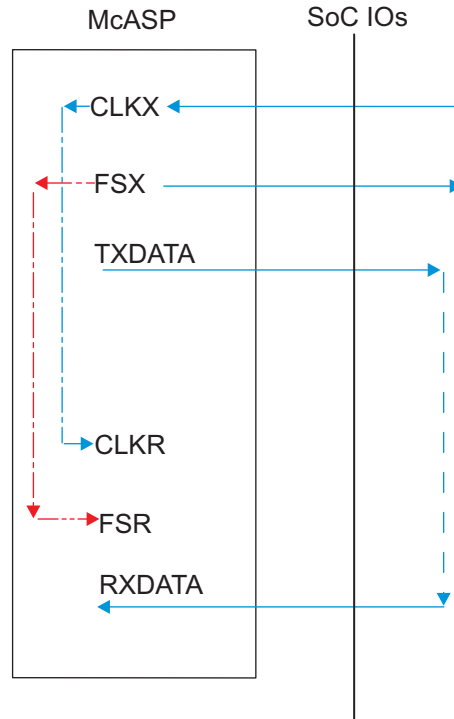
7-48. McASP1-8 CI-FO- - SYNC Mode
