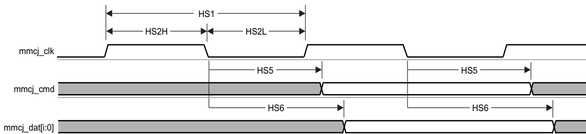
SPRS906_TIMING_MMC3_10
