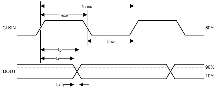
図 5-1. Digital Interface Timing
