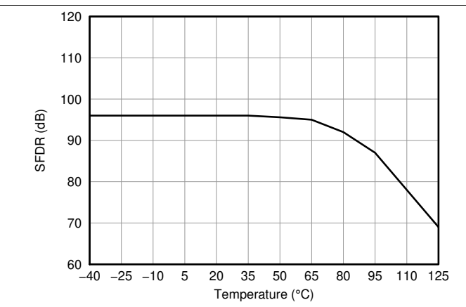
Figure 29. Spurious-Free Dynamic Range vs Temperature
