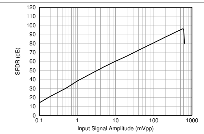
Figure 31. Spurious-Free Dynamic Range vs Input Signal Amplitude
