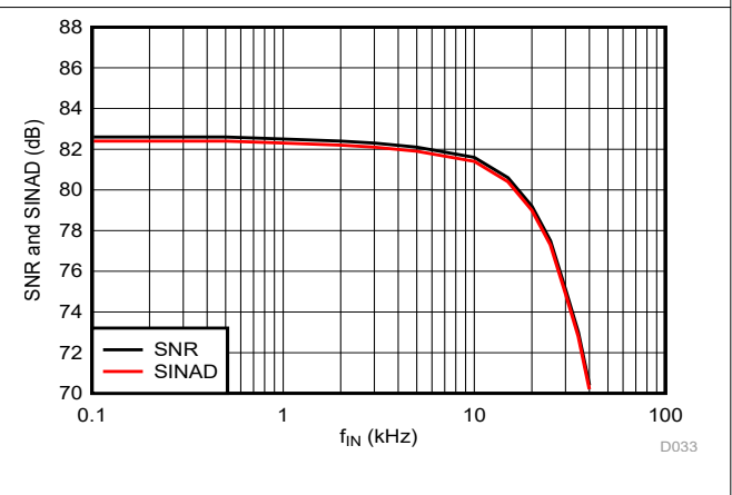
FIG 6-21. Signal-to-Noise Ratio and Signal-to-Noise + Distortion vs Input Signal Frequency
