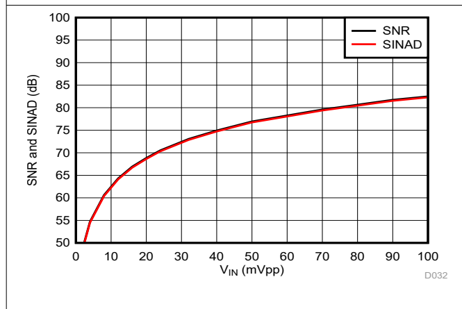
FIG 6-22. Signal-to-Noise Ratio and Signal-to-Noise + Distortion vs Input Signal Amplitude
