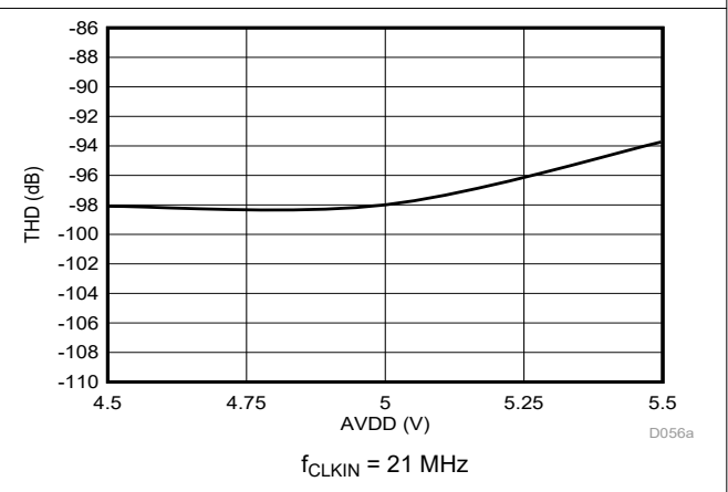
FIG 6-23. Total Harmonic Distortion vs High-Side Supply Voltage (5 V, nom)
