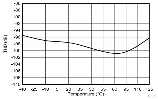
6-25. Total Harmonic Distortion vs Temperature
