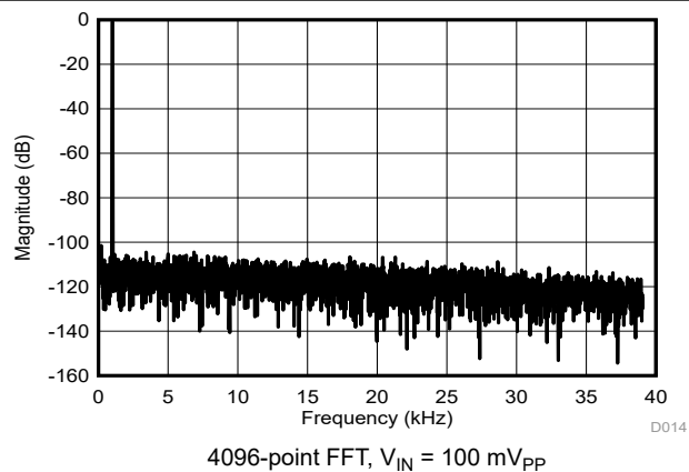
6-34. Frequency Spectrum With 1-kHz Input Signal
