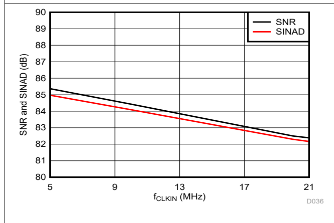
FIG 6-20. Signal-to-Noise Ratio and Signal-to-Noise + Distortion vs Clock Frequency
