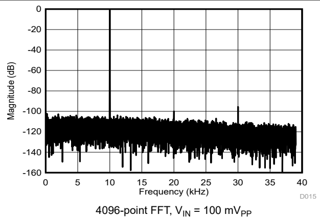
6-35. Frequency Spectrum With 10-kHz Input Signal
