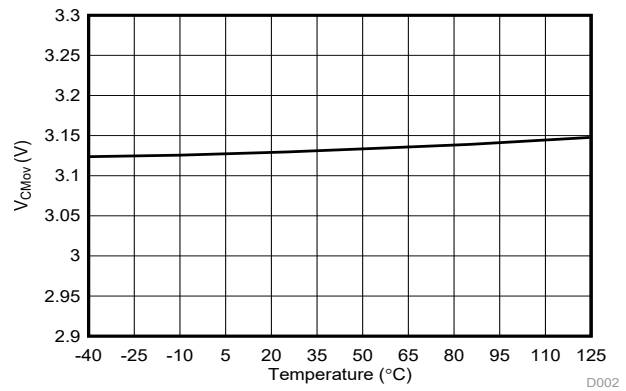
Figure 6-7. Common-Mode Overtolerance Detection Level vs Temperature
