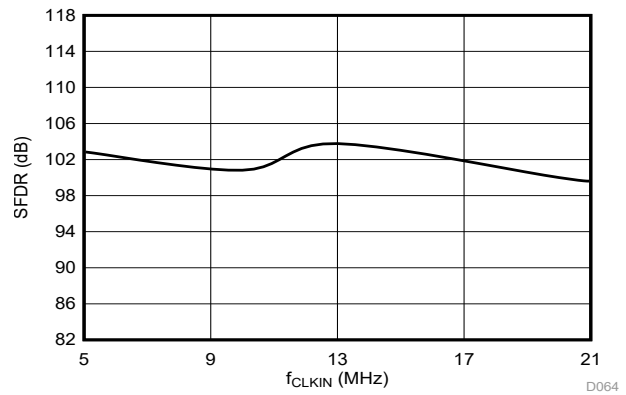
6-31. Spurious-Free Dynamic Range vs Clock Frequency
