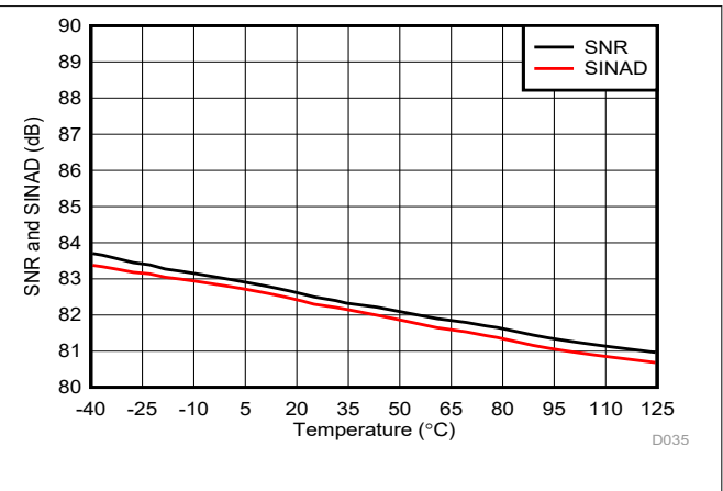
FIG 6-19. Signal-to-Noise Ratio and Signal-to-Noise + Distortion vs Temperature
