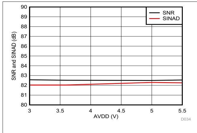
FIG 6-18. Signal-to-Noise Ratio and Signal-to-Noise + Distortion vs High-Side Supply Voltage
