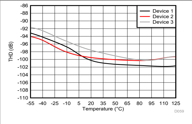
6-25. Total Harmonic Distortion vs Temperature
