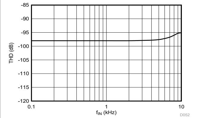
6-27. Total Harmonic Distortion vs Input Signal Frequency
