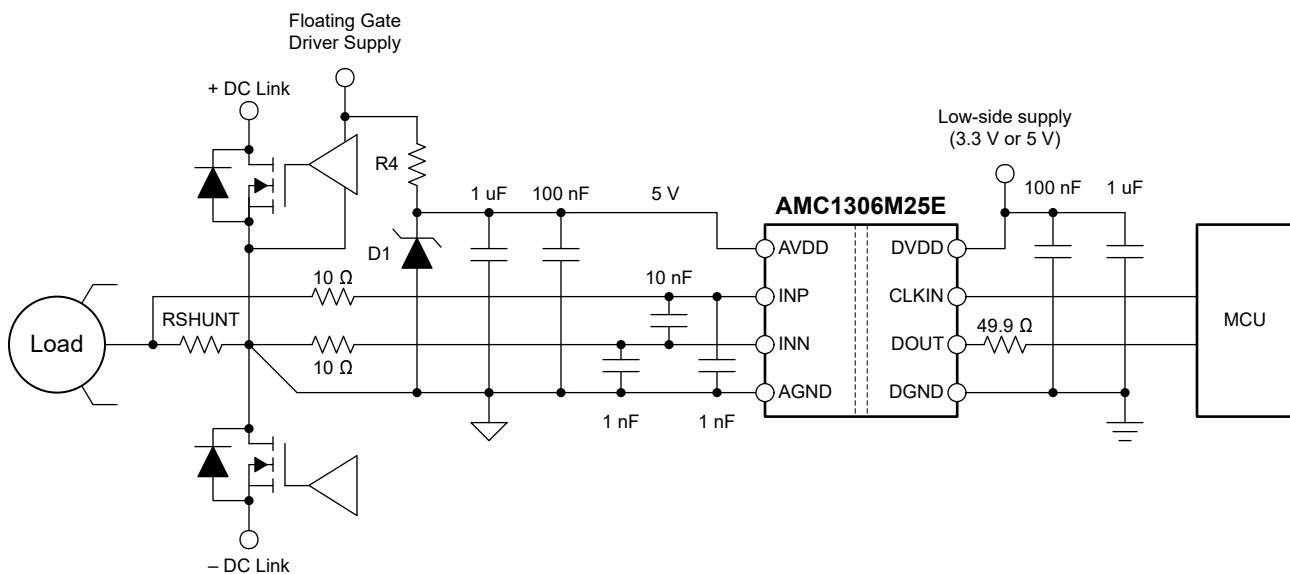
図 8-1. Using the AMC1306M25E for Current Sensing in a Typical Application
