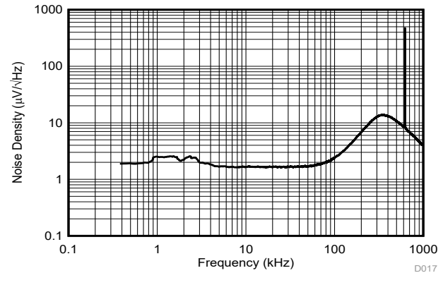
Figure 6-26. Input-Referred Noise Density vs Frequency
