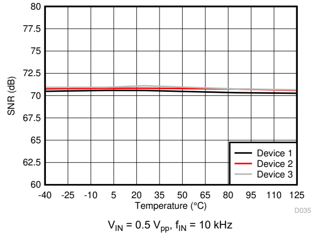
6-24. Signal-to-Noise Ratio vs Temperature
