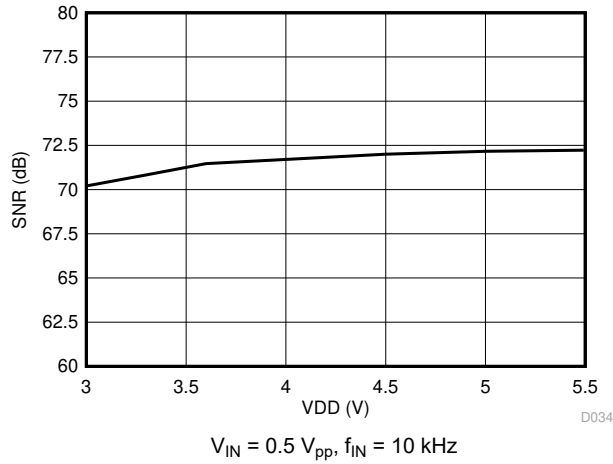
6-23. Signal-to-Noise Ratio vs Supply Voltage
