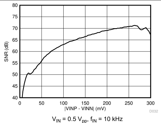
6-22. Signal-to-Noise Ratio vs Input Voltage
