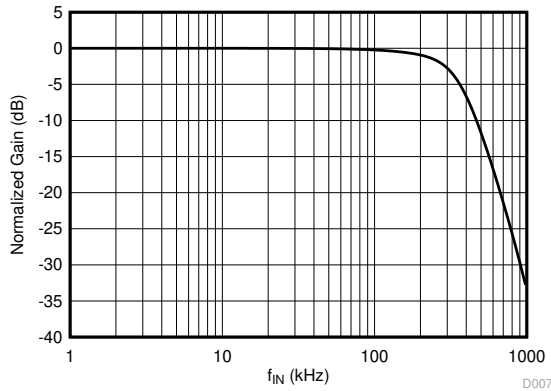
6-11. Normalized Gain vs Input Frequency
