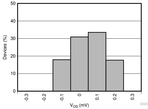
6-17. Offset Error Histogram
