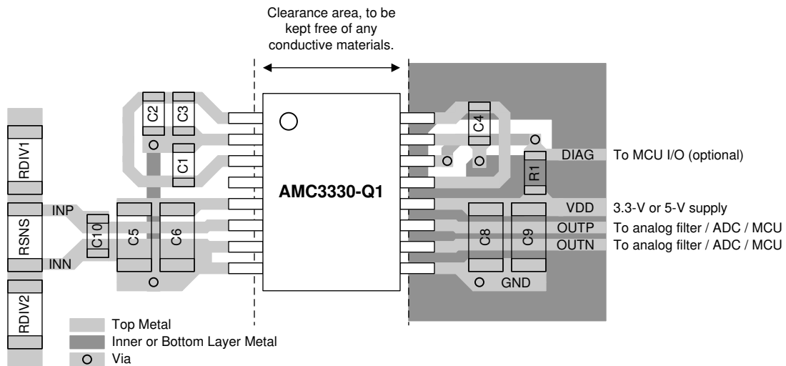
☒ 10-1. Recommended Layout of the AMC3330-Q1
