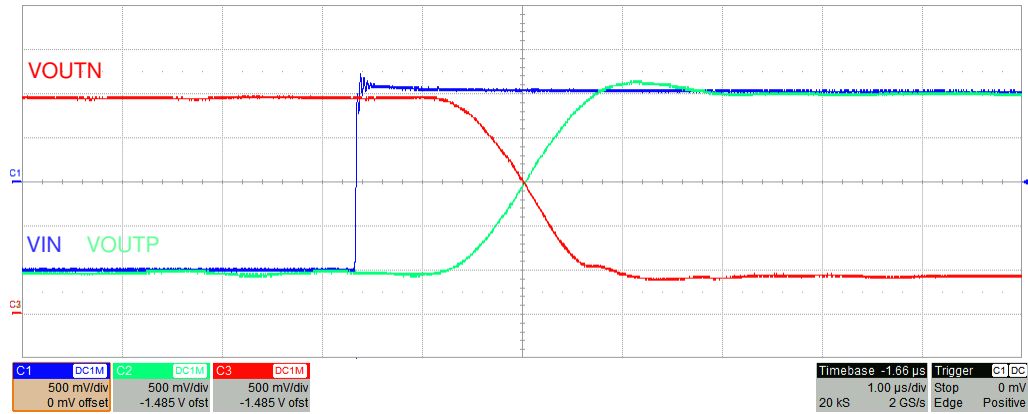
Figure 8-4. Step Respose of the AMC3330-Q1
