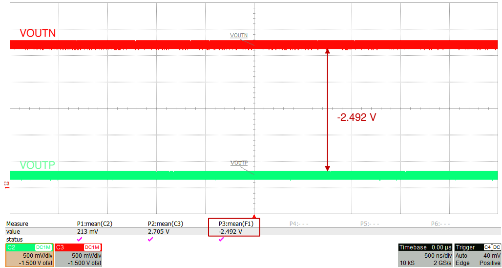
7-4. Typical Negative Clipping Output of the AMC3330-Q1
