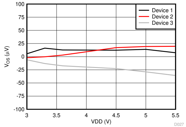
6-18. Offset Error vs Supply Voltage
