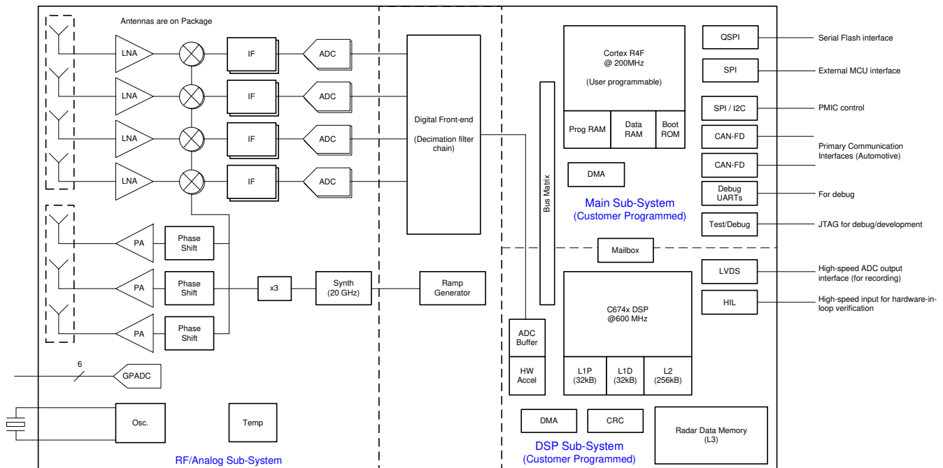
9-1. Functional Block Diagram
