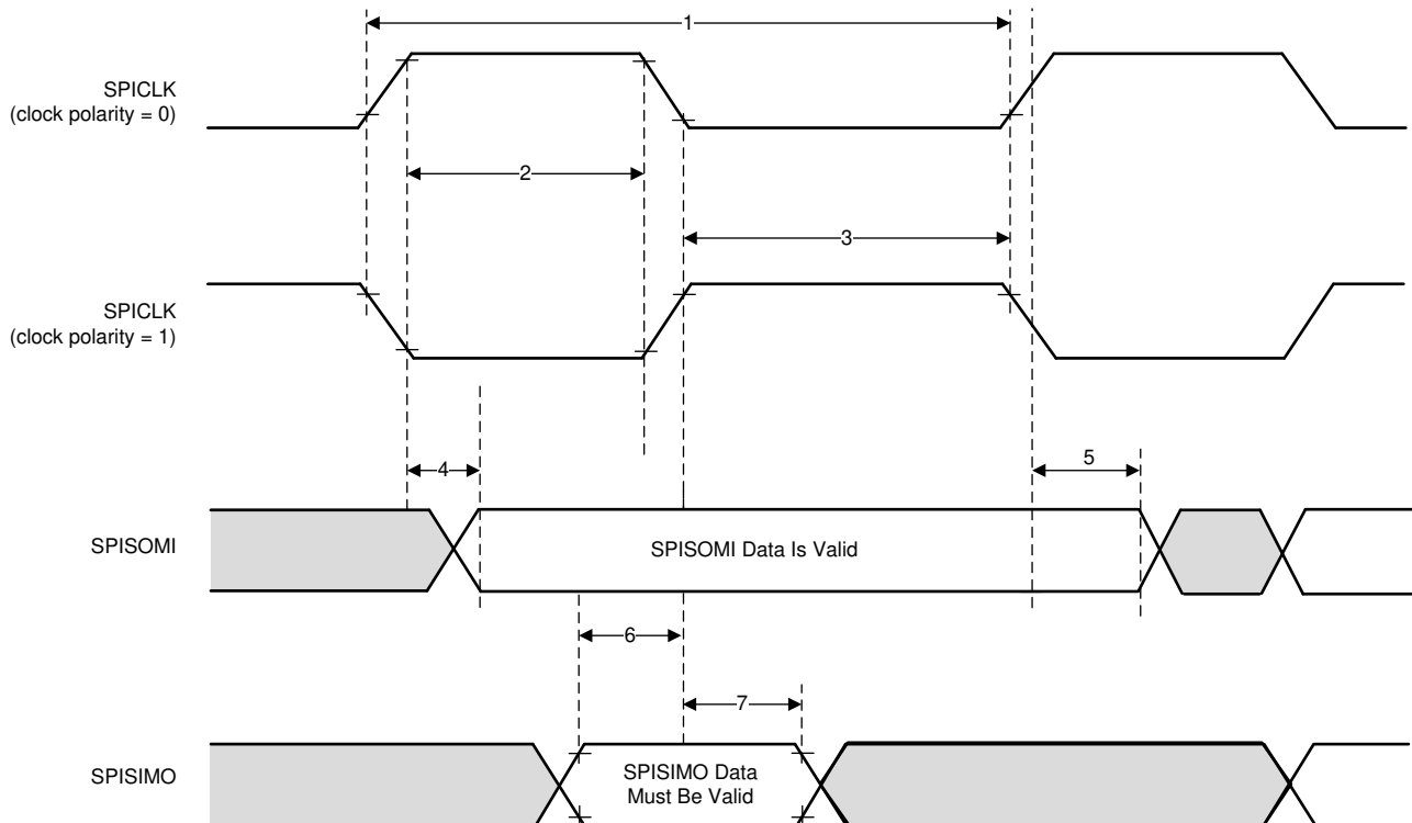
8-10. SPI Peripheral Mode External Timing (CLOCK PHASE = 0)
