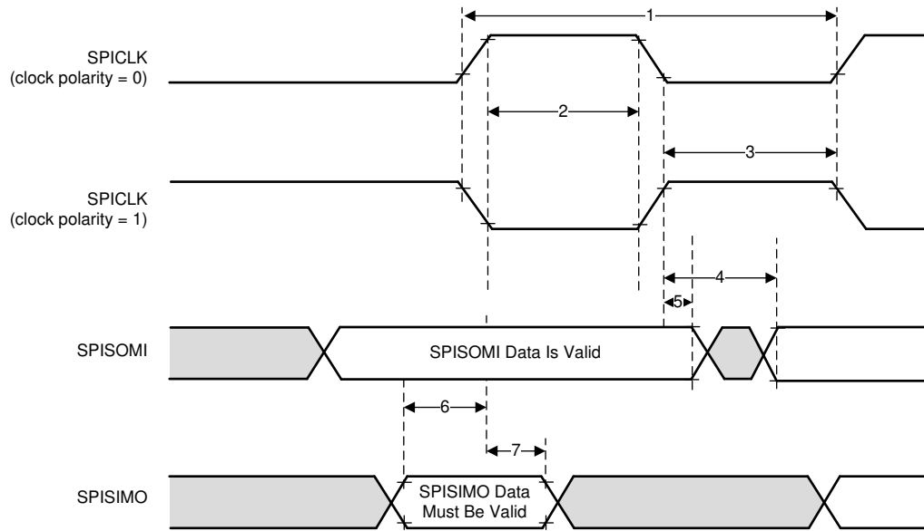
8-11. SPI Peripheral Mode External Timing (CLOCK PHASE = 1)
