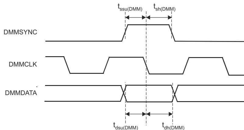
8-21. DMMDATA Timing
