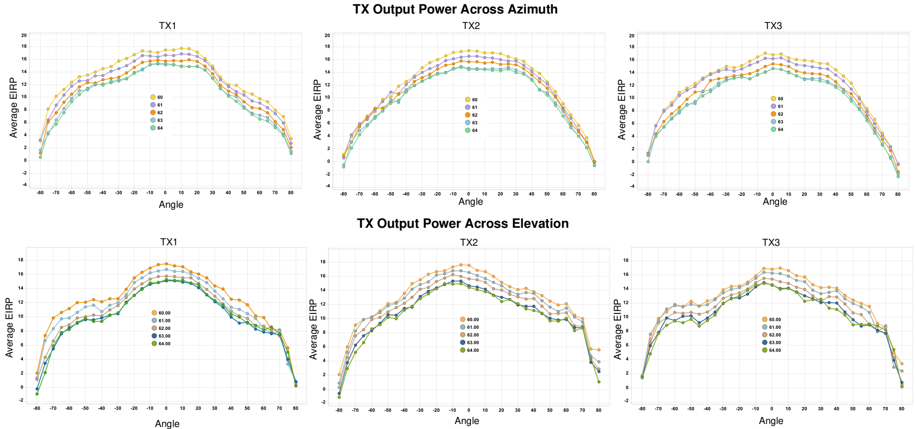
8-2. Transmitter Antenna Radiation Pattern
