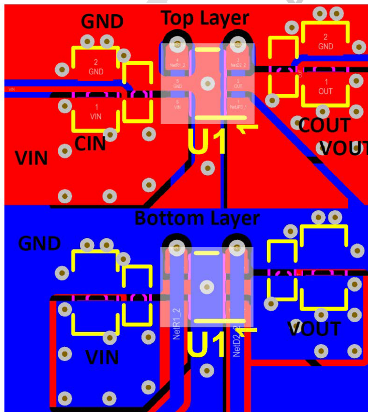
⊗ 29. Board Layout
