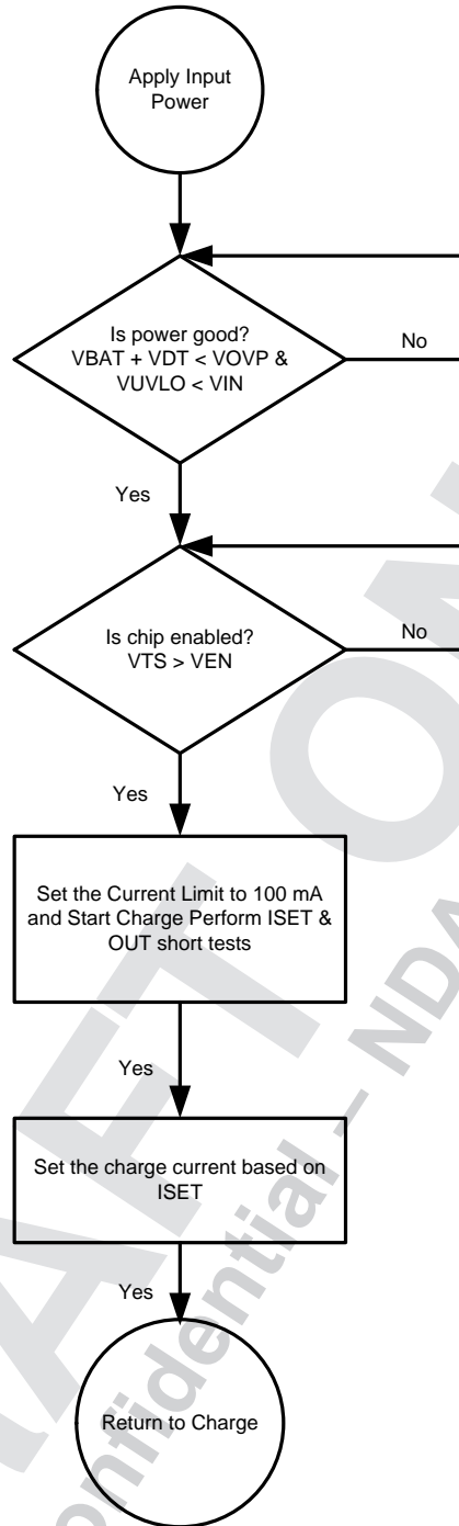
Fig 7. bq21040 Power-Up Flow Diagram
