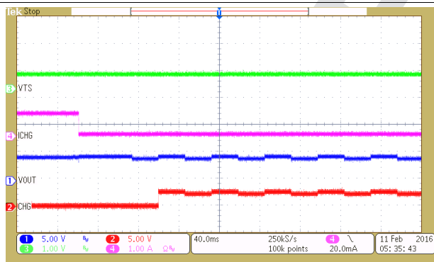
19. Battery Removal - GND Removed 1st, 42-Ω Load
