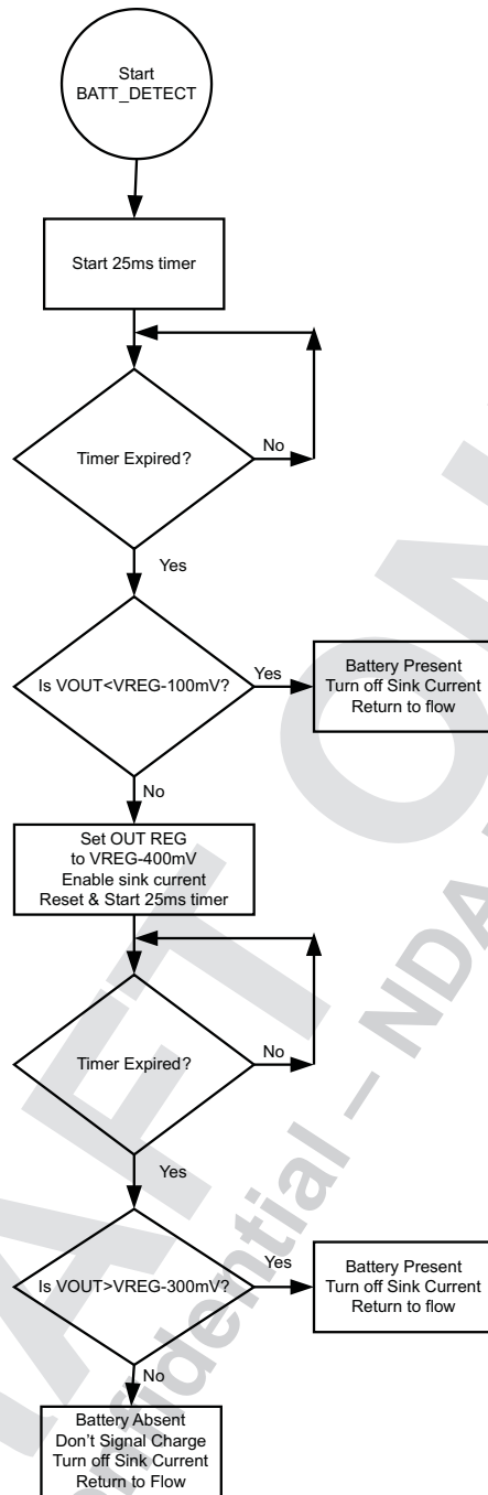
9. Battery Detect Routine (bq21040)
