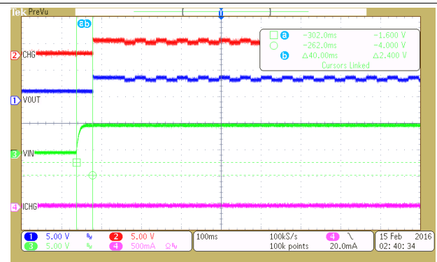
18. Power-Up Timing with No Battery and No Load - Battery Detection
