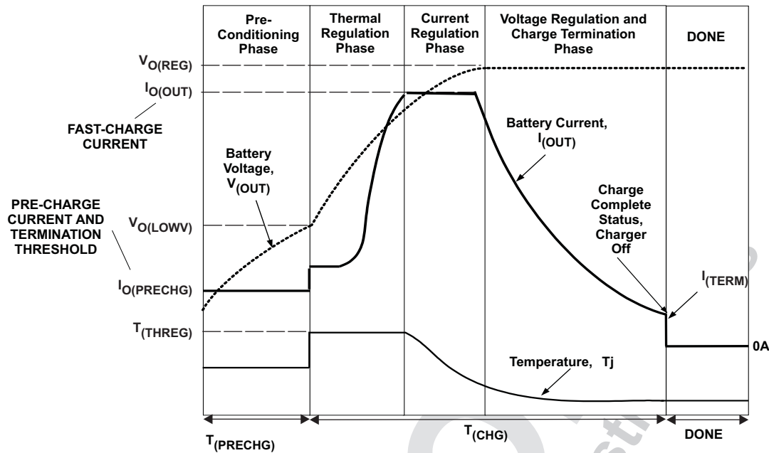
✎ 5. Charging Profile With Thermal Regulation
