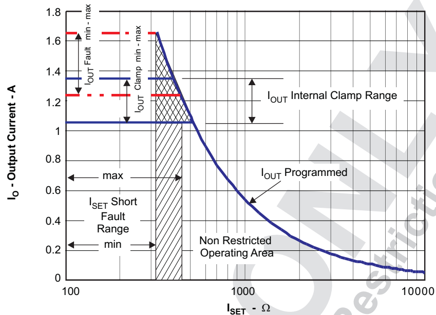
Fig. 8. Programmed/Clamped Out Current
