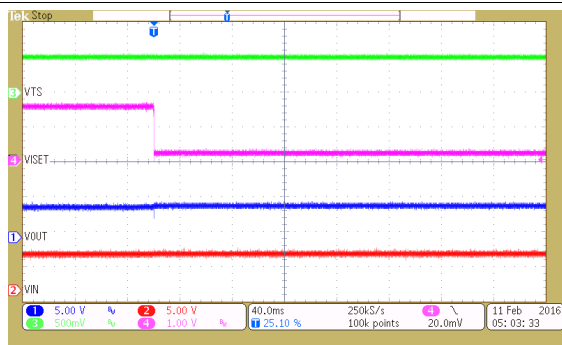
17. TS Enable and Disable
