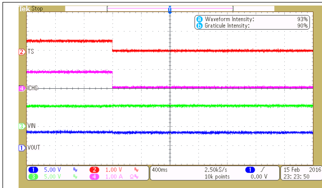
17. TS Enable and Disable
