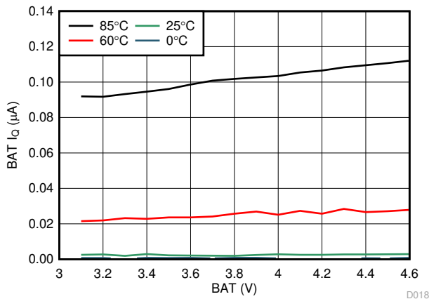
Figure 8-5. Ship Mode BAT, I Q
