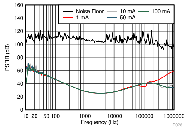
Figure 8-14. LS/LDO PSRR vs Frequency
