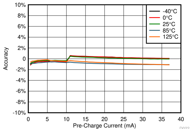
Figure 8-11. Pre-Charge Accuracy vs Pre-Charge Current
