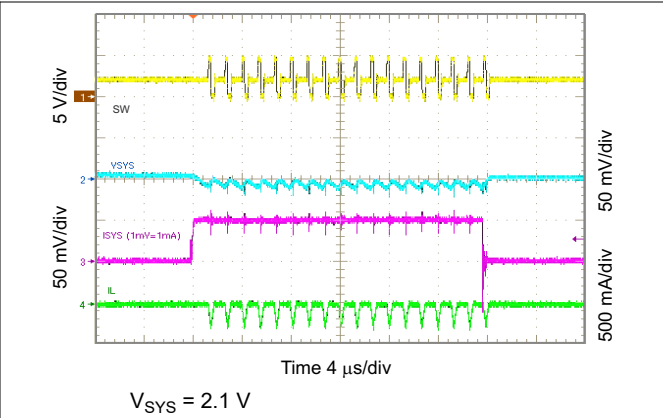
Figure 10-35. 2.1 V SYS Load Transient, 0 to 50 mA
