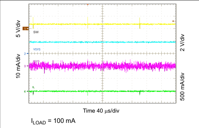
Figure 10-27. Light Load Operation Showing SW
