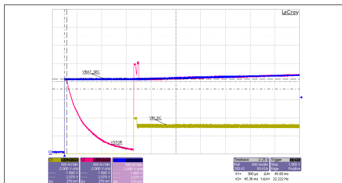
Sourcemeter with V_{SOURCE} = 1.0\text{ V} and compliance of 8.5 mA subsequently applied to V_{IN\_DC} V_{BAT\_SEC} = 0.1\text{ F} capacitor charged to 2.0 V Resistance on V_{STOR} = 100\text{ k}\Omega
