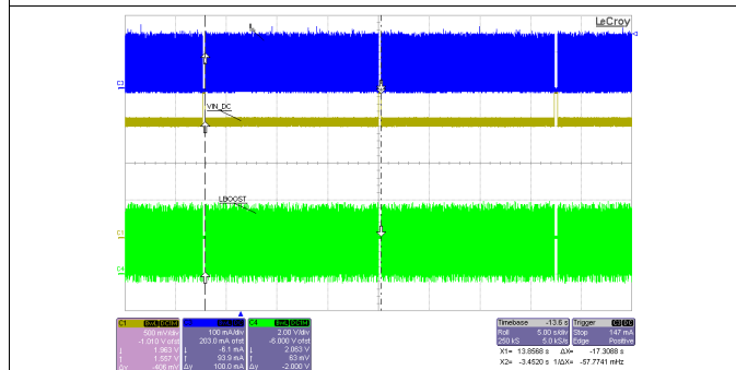
V_{IN\_DC} = sourcemeter with V_{SOURCE} = 2.0\text{ V} and compliance of 43 mA V_{BAT\_SEC} = sourcemeter with V_{SOURCE} = 3.0\text{ V} and compliance of 1 A
