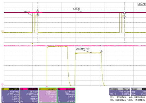
VIN_DC = sourcemeter with V_{\text{SOURCE}} = 2.0 \text{ V} and compliance of 43 mA VBAT_SEC = sourcemeter with V_{\text{SOURCE}} = 4.0 \text{ V} and compliance of 1 A
