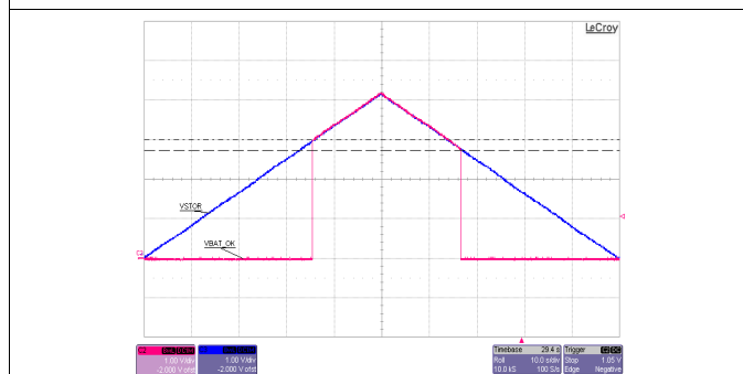
V_{IN\_DC} = 1.5\text{ V} with 75\ \Omega series resistance No storage element on V_{BAT\_SEC} or V_{BAT\_PRI} V_{STOR} artificially ramped from 0 V to 4.2 V to 0 V using a power amp driven by a function generator
