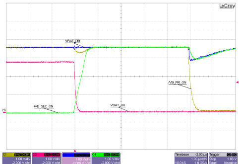
VIN_DC = 1.5 V with 75 Ω series resistance; VBAT_PRI = 3.6 V power supply 0.5 F super capacitor on VBAT_SEC; 1kΩ load on output of MUX FETs (VOR) VSTOR artificially ramped from 4.2 V to 0 V using a function generator
