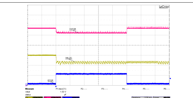
V_{IN\_DC} = 1.5\text{ V} with 75\ \Omega series resistance V_{BAT} = 4.2\text{ V} charged 0.5 F capacitor R(V_{STOR}) = open to 84\ \Omega to open
