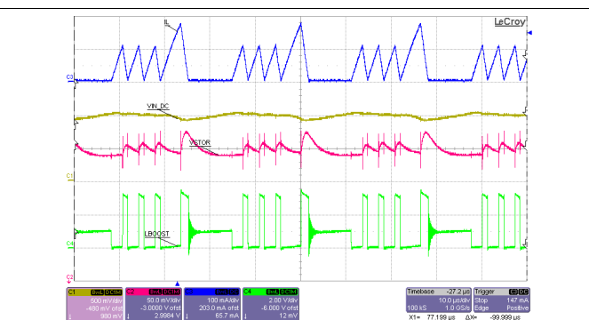
V_{IN\_DC} = sourcemeter with V_{SOURCE} = 2.0\text{ V} and compliance of 43 mA V_{BAT\_SEC} = sourcemeter with V_{SOURCE} = 3.0\text{ V} and compliance of 1 A I_L = inductor current
