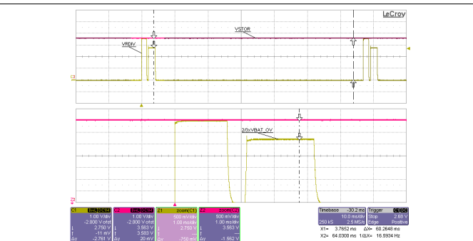
V_{IN\_DC} = sourcemeter with V_{SOURCE} = 2.0\text{ V} and compliance of 43 mA V_{BAT\_SEC} = sourcemeter with V_{SOURCE} = 3.6\text{ V} and compliance of 1 A
