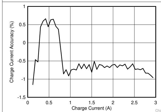
8-3. Charge Current Accuracy
