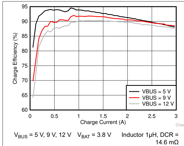
8-1. Charge Efficiency
