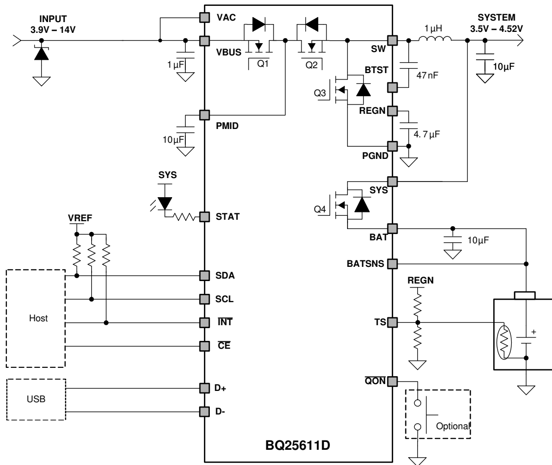
10-1. BQ25611D Application Diagram
