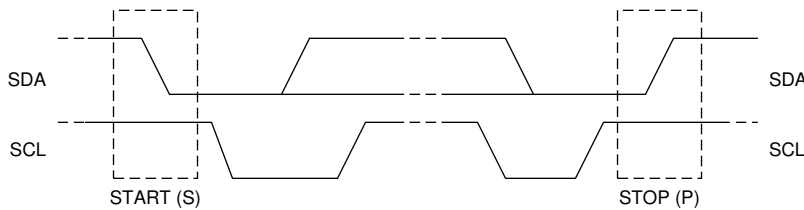
9-9. TS START and STOP conditions
