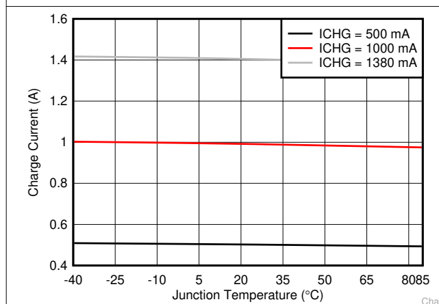
8-5. Charge Current vs Junction Temperature
