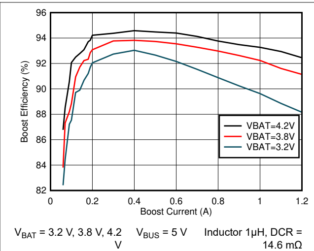
8-2. Boost Efficiency
