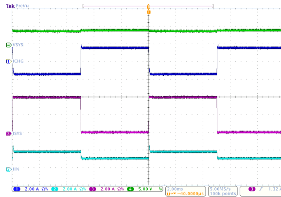
10-6. System Load Transient Response
