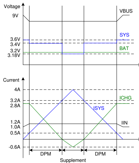
9-2. DPM Response
