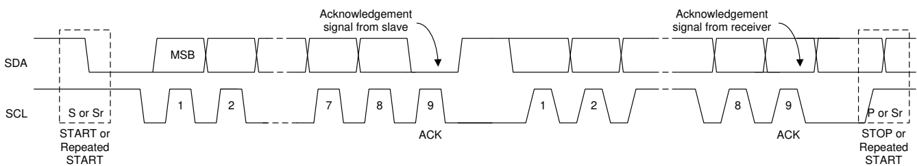
9-10. Data Transfer on the I 2 C Bus
