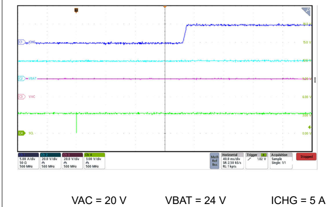
9-5. Charge Enable via I 2 C with 5-A ICHG
