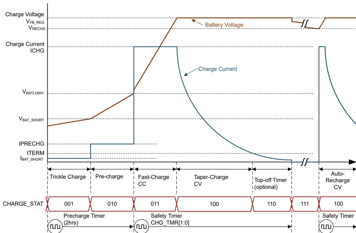
図 8-3. Typical Li-Ion Battery Charging Profile
