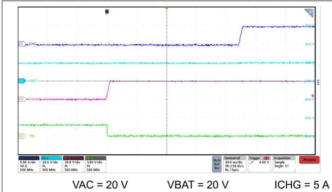
9-3. VAC Plug-In Power Up with 5-A ICHG
