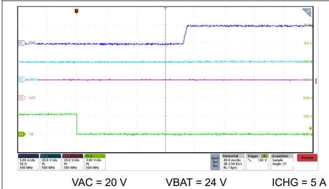
9-7. Charge Enable via \overline{\text{CE}} Pin with 5-A ICHG
