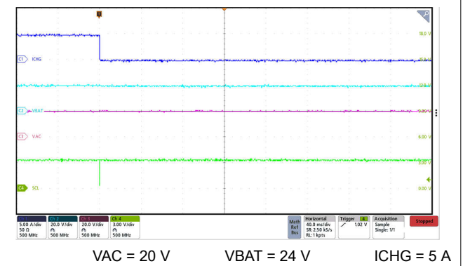
9-6. Charge Disable via I 2 C with 5-A ICHG
