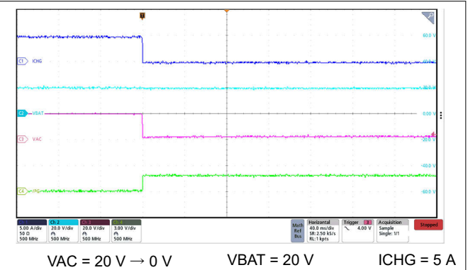
9-4. VAC Un-plug Power Down with 5-A ICHG
