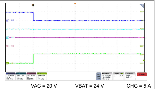
9-8. Charge Disable via \overline{\text{CE}} Pin with 5-A ICHG
