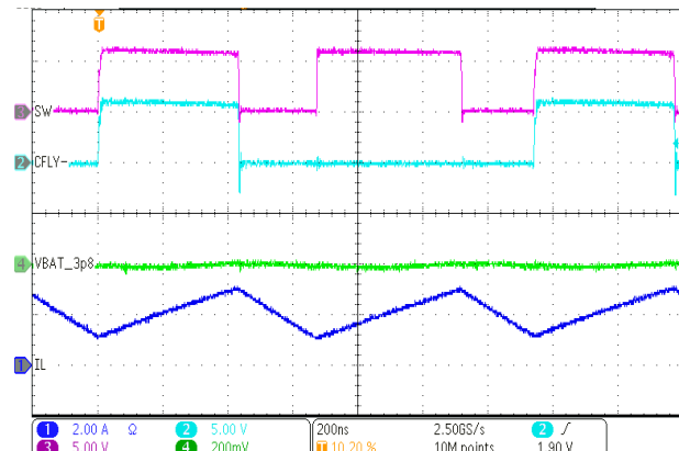
VBUS = 12 V, VBAT = 3.8 V, ICHG = 2 A (D < 50%)
