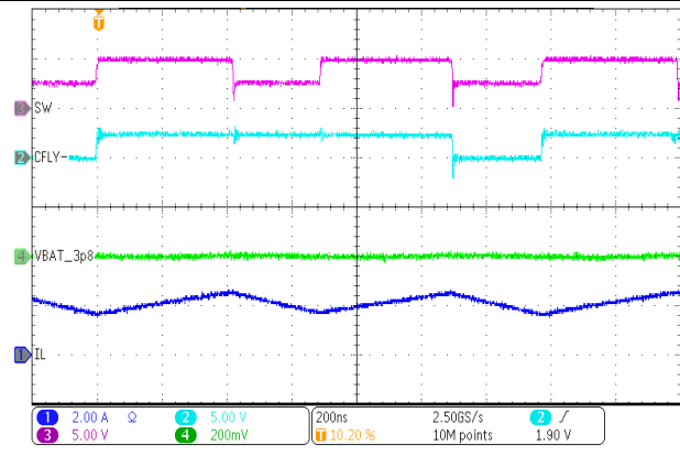
VBUS = 5 V, VBAT = 3.8 V, ICHG = 2 A, (D > 50%)
