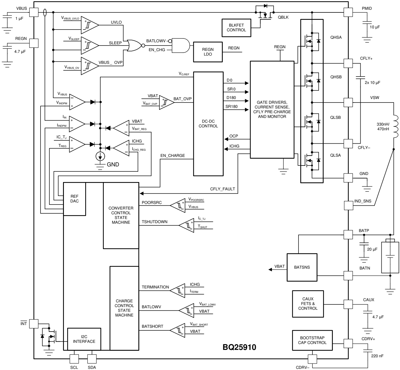
图 13. BQ25910 I 2 C Controlled Functional Block Diagram
