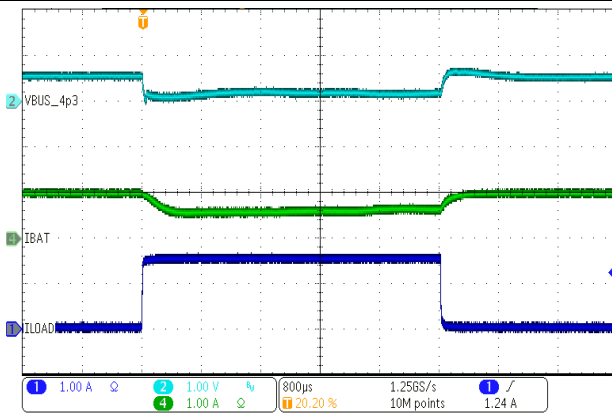
VBAT = 4.1 V, VINDPM = 4.3 V
