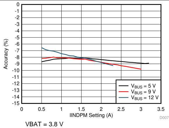
9. Input Current Limit Accuracy vs I 2 C IINDPM Setting
