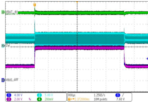
VBUS = 5 V \rightarrow 12 V \rightarrow 5 V, VBAT = 4 V, ICHG = 1 A CH 1 = VBUS, CH2 = SW, CH3 = CFLY differential, CH4 = VBAT
