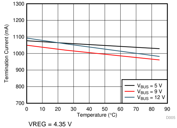
8. Termination Current vs Temperature
