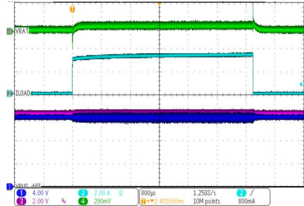
VBUS = 12 V, VBAT = 4.35 V, ICHG = 4 A, IBAT = 1 A \rightarrow 4 A \rightarrow 1 A CH 1 = VBUS, CH2 = ILOAD, CH3 = CFLY differential, CH4 = VBAT
