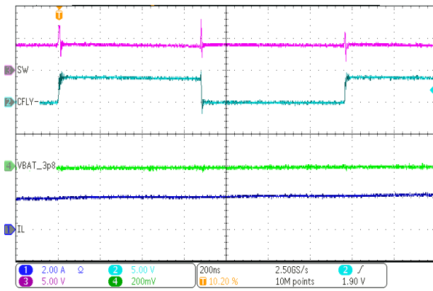
VBUS = 8 V, VBAT = 3.8 V, ICHG = 2 A, (D approx. 50%)
