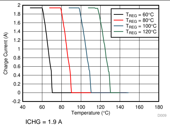
12. Charge Current vs Temperature
