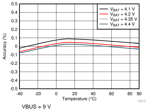
7. Battery Voltage Regulation Accuracy vs Temperature
