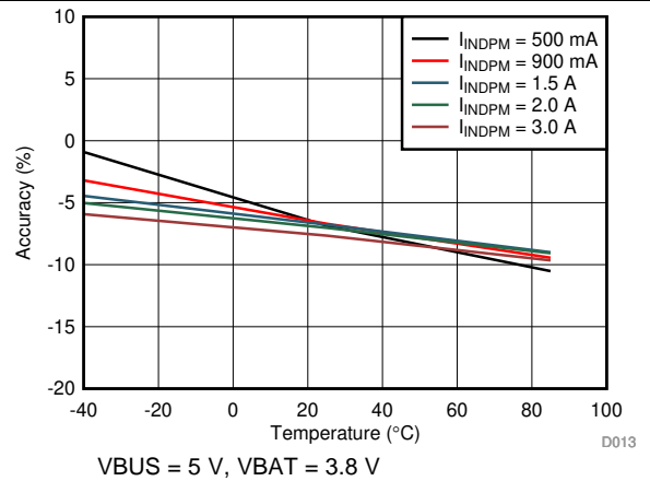
10. Input Current Limit Accuracy vs Temperature
