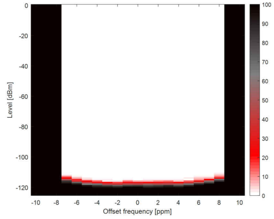
8-20. Narrowband, 9.6 kbps \pm 2.4 kHz deviation, 2-GFSK, 868 MHz, 17.1 kHz RX Bandwidth
