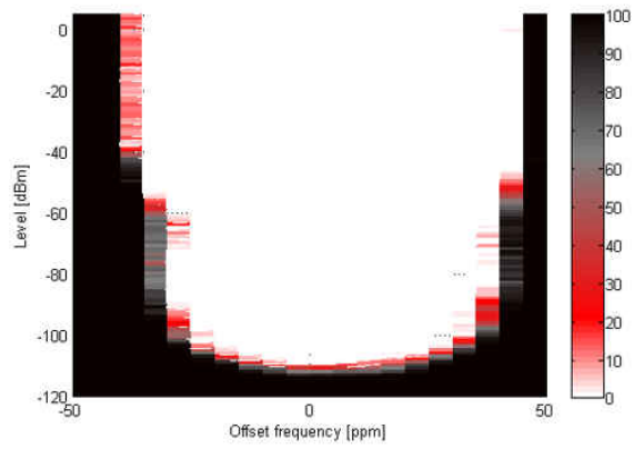
8-19. 802.15.4, 50 kbps, \pm 25 kHz deviation, 2-GFSK, 100 kHz RX Bandwidth
