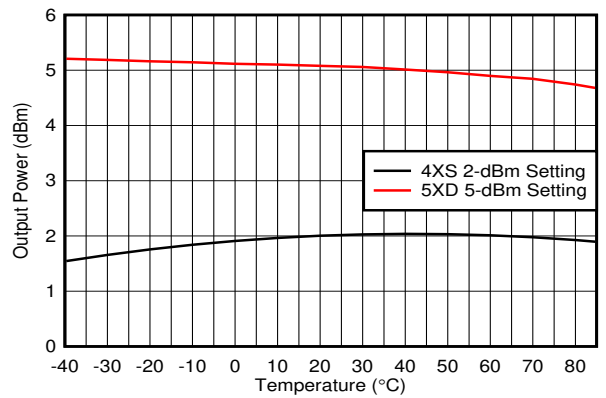
8-7. TX Output Power vs Temperature
