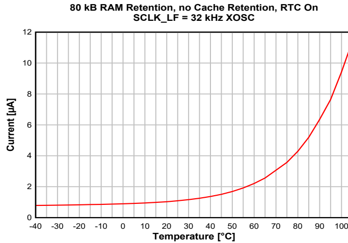
7-5. Standby Mode (MCU) Current vs. Temperature
