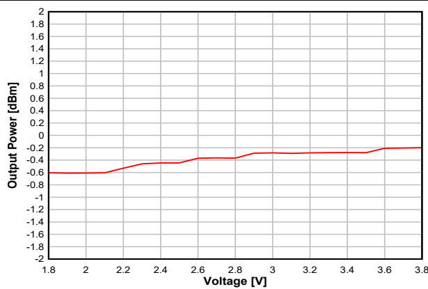
7-25. Output Power vs. Supply Voltage (VDDS) (BLE 1 Mbps, 2.44GHz, 0dBm)
