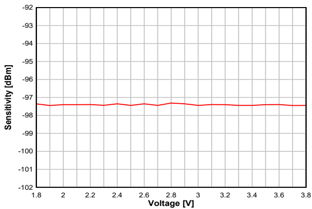
7-19. Sensitivity vs. Supply Voltage (VDD5) (BLE 1Mbps, 2.44GHz, DCDC Off)
