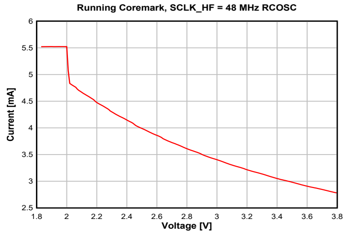
7-4. Active Mode (MCU) Current vs. Supply Voltage (VDD5)
