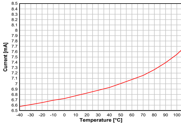
☒ 7-6. RX Current vs. Temperature (BLE 1Mbps, 2.44GHz)
