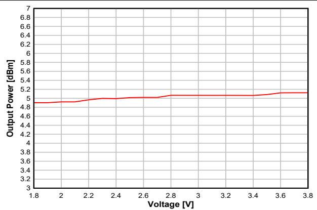
7-26. Output Power vs. Supply Voltage (VDDS) (BLE 1 Mbps, 2.44GHz, +5dBm)
