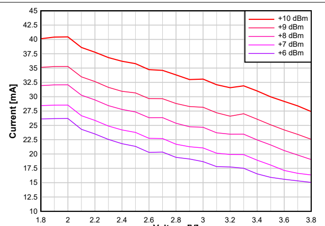
8-13. TX Current vs. Supply Voltage (VDD5) (BLE 1 Mbps, 2.44 GHz, +10 dBm PA)
