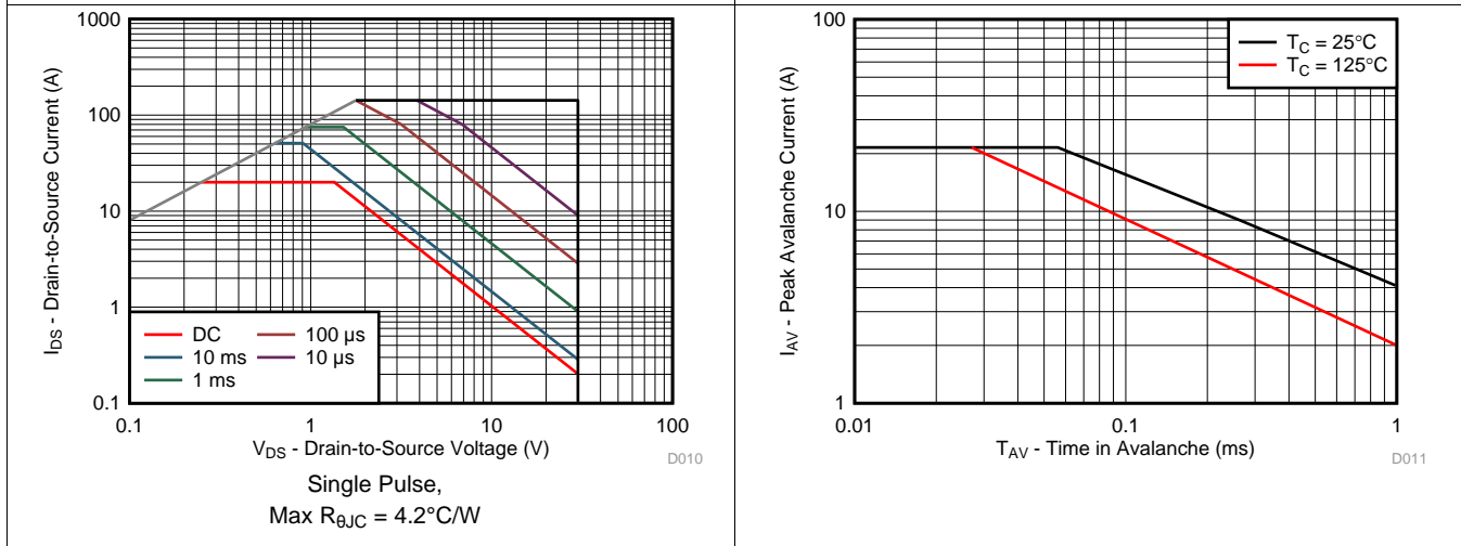
Figure 10. Maximum Safe Operating Area (SOA)
