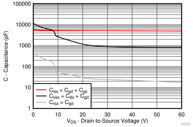
4-5. Capacitance
