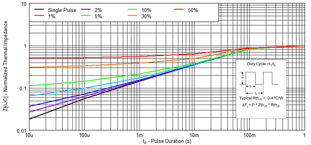
4-1. Transient Thermal Impedance
