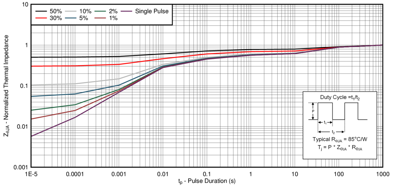
5-1. Transient Thermal Impedance
