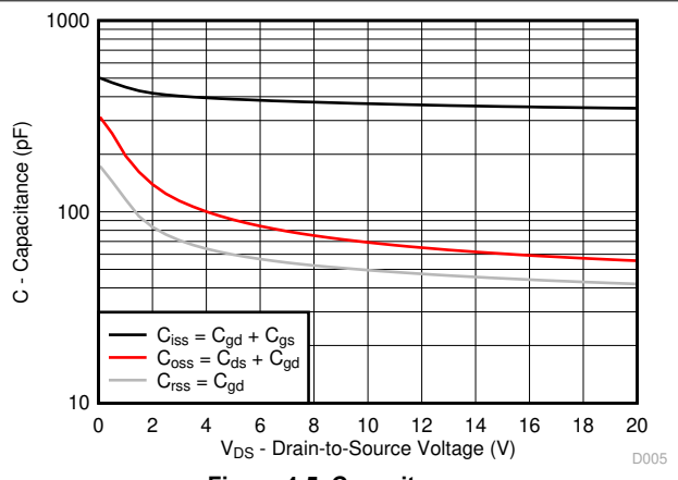
Figure 4-5. Capacitance
