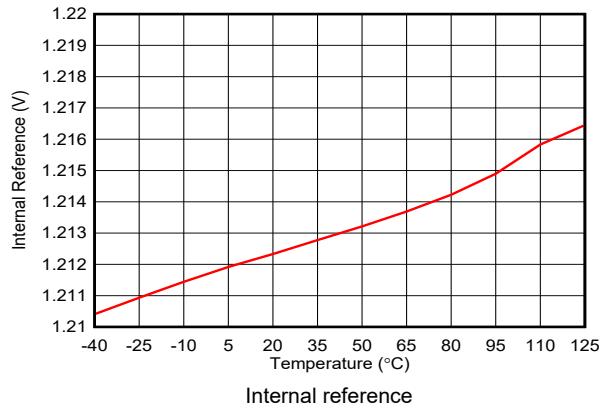
6-54. Internal Reference vs Temperature
