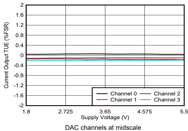
6-39. Current Output TUE vs Supply Voltage
