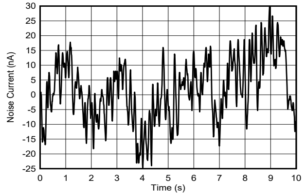
6-50. Current Output Flicker Noise
