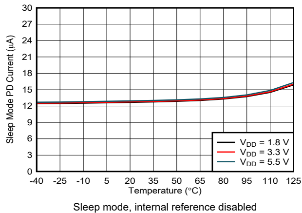
6-56. Power-Down Current vs Temperature
