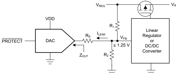
图 7-9. High-Impedance (Hi-Z) Output and \overline{\text{PROTECT}} Input
