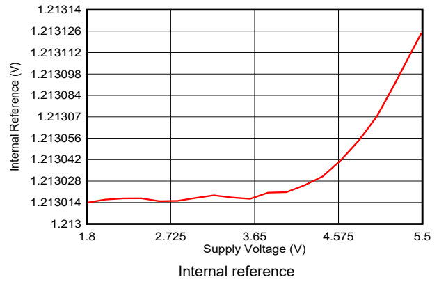
6-55. Internal Reference vs Supply Voltage
