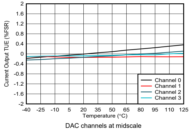
6-38. Current Output TUE vs Temperature
