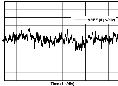
80. Internal Reference Noise, 0.1 Hz to 10 Hz
