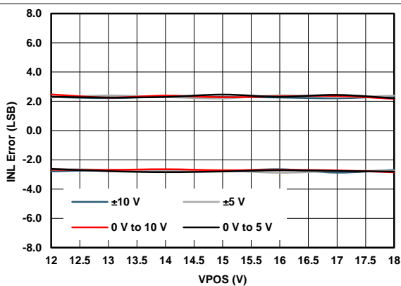
56. VOUT Linearity Error vs Power Supplies
