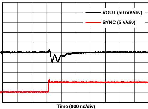
⊠ 62. VOUT Full-Scale Settling Time, Rising Edge
