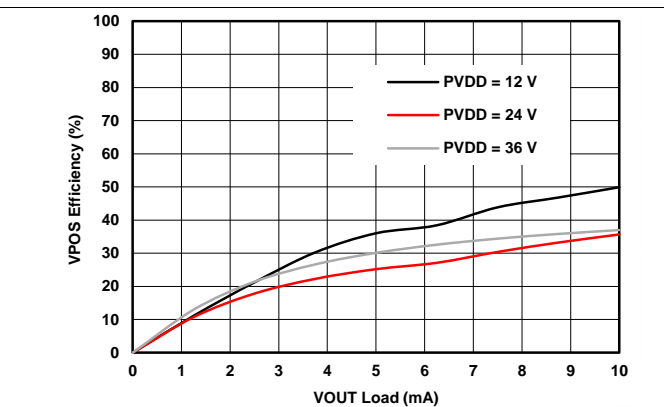
95. VPOS Efficiency (VOUT Mode) vs Load Current
