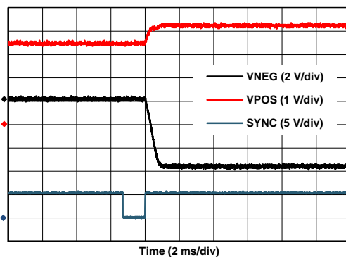
84. Buck-Boost Converter Power-On (VOUT Mode)
