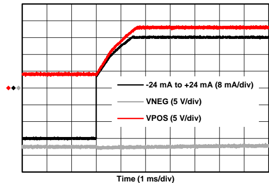
IOUT R L = 625 Ω
