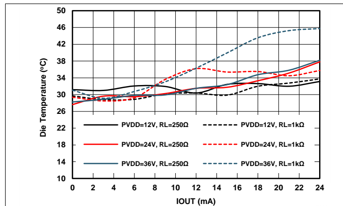
94. Internal Die Temperature (IOUT Mode) vs Load Current
