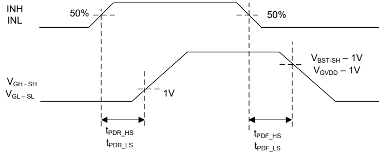
☒ 6-1. Gate Driver Propagation Delay Timing Diagram
