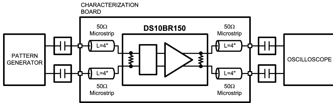
FIGURE 5. Jitter Measurements Test Circuit
