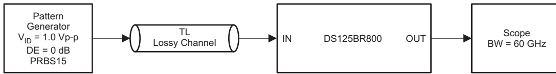
Figure 10. Test Setup Connections Diagram
