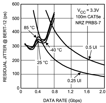
Residual Jitter as a Function of Data Rate and Temperature for the Chipset with 100m CAT5e
