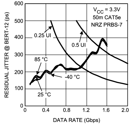
Residual Jitter as a Function of Data Rate and Temperature for the Chipset with 50m CAT5e
