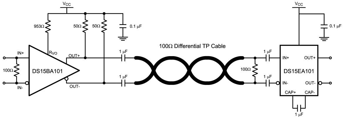
Cable Extender Chipset Connection Diagram for 100 Differential Cables
