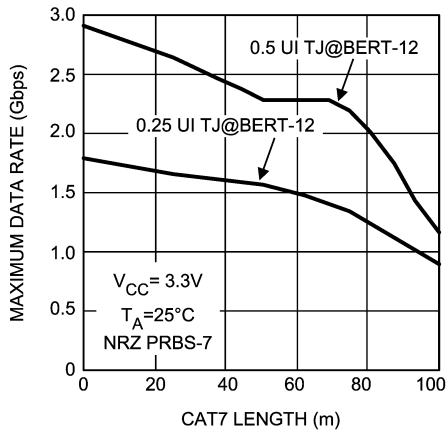
Maximum Data Rate as a Function of CAT7 (Siemon CAT7 Tera) Length
