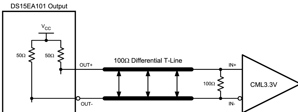
Typical DS15EA101 Output DC-Coupled Interface to a CML Receiver
