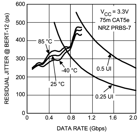
Residual Jitter as a Function of Data Rate and Temperature for the Chipset with 75m CAT5e
