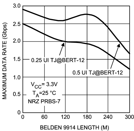
Maximum Data Rate as a Function of 50 Coaxial (Belden 9914) Length
