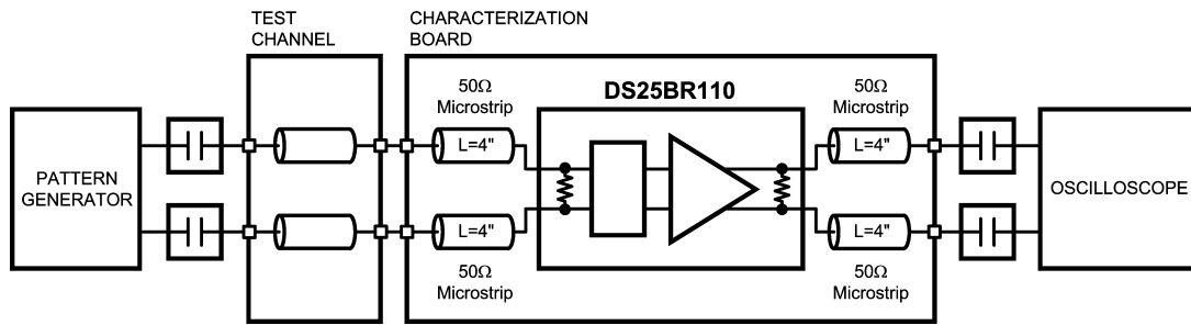
FIGURE 5. Equalization Performance Test Circuit
