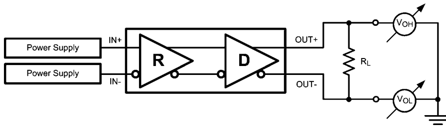
FIGURE 1. Differential Driver DC Test Circuit
