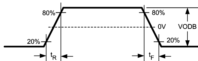
FIGURE 2. Driver Output Transition Time
