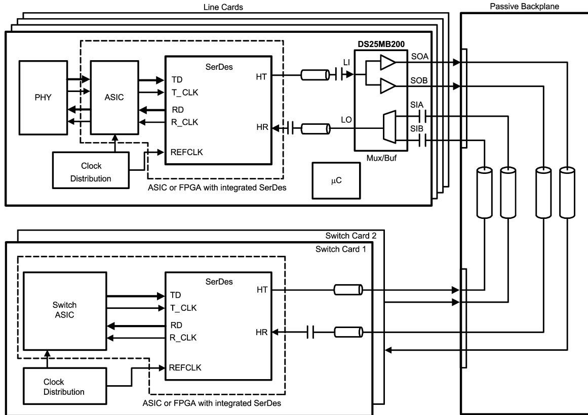
FIGURE 7. Application Diagram (showing data paths of port 0)
