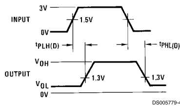
FIGURE 1. Propagation Delay Differential Input to Output
