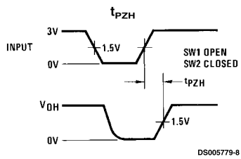
FIGURE 2. Propagation Delay TRI-STATE Control Input to Output
