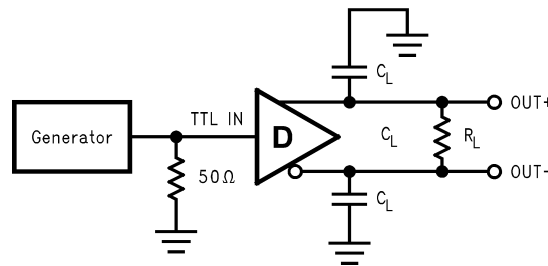
7-3. Differential Driver Propagation Delay and Transition Time Test Circuit
