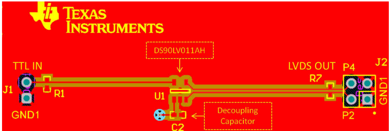
11-10. Example DS90LV011AH Layout
