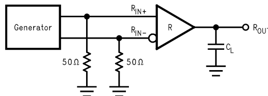
Figure 14. Receiver Propagation Delay and Transition Time Test Circuit
