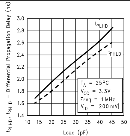
Figure 10. Differential Propagation Delay vs Load
