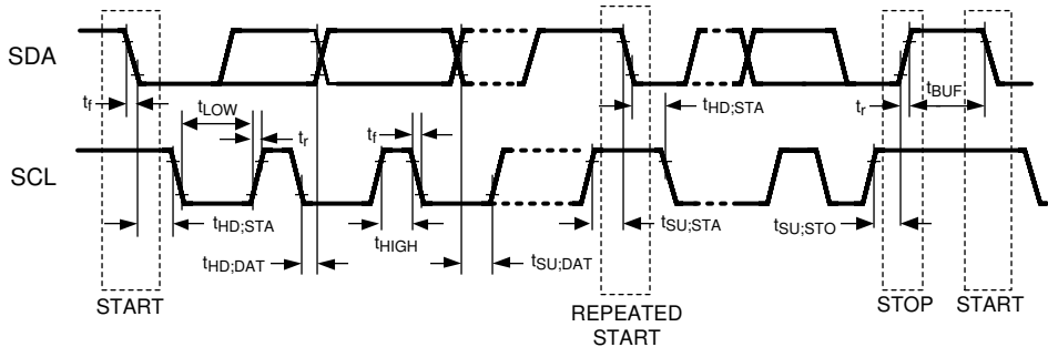
6-11. Serial Control Bus Timing Diagram
