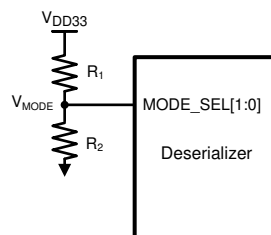
☒ 7-16. MODE_SEL[1:0] Connection Diagram
