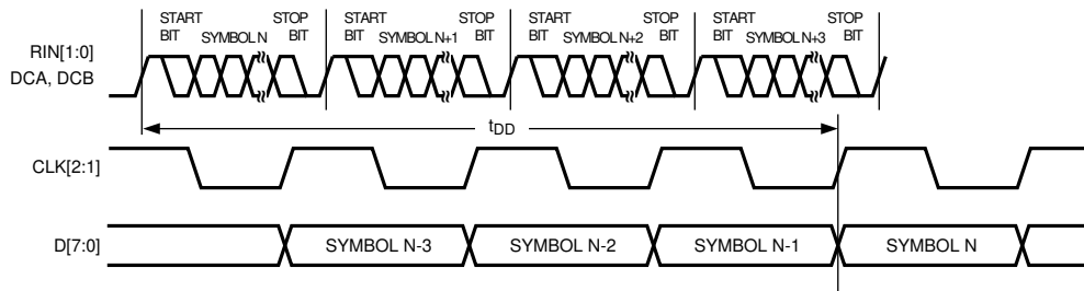
6-4. Latency Delay
