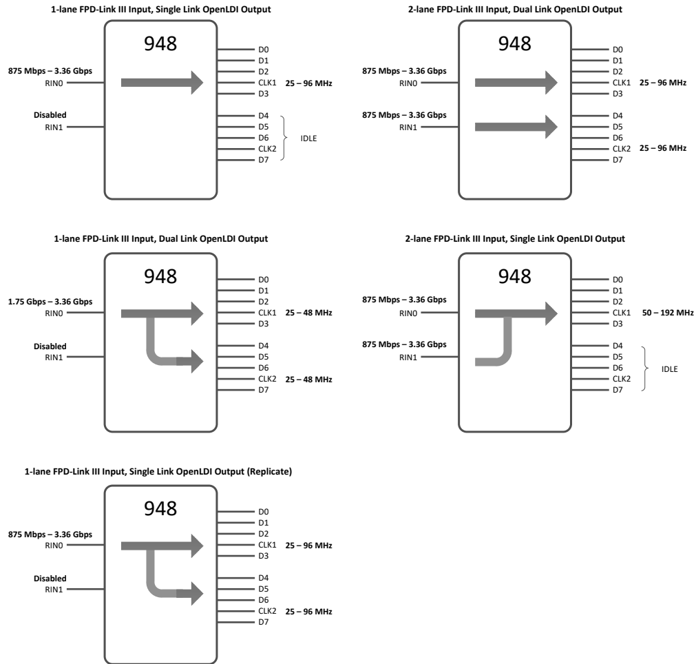
☒ 7-15. Data-Path Configurations
