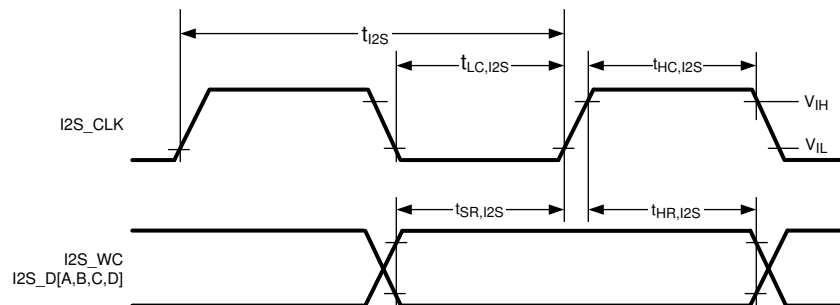
6-12. I2S Timing
