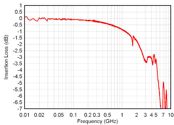
Figure 6-17. Insertion Loss
