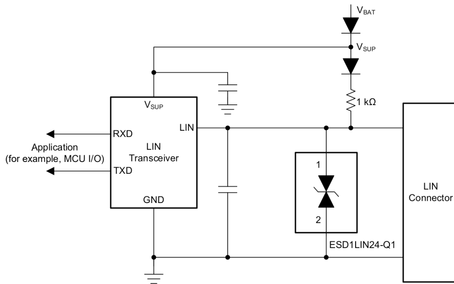
图 8-1. Typical Application
