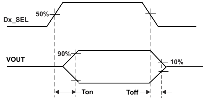
图 7-1. Select to Switch T on and T off
