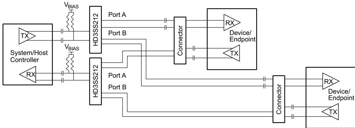
9-3. AC Coupling Capacitors on Both Sides of Switch
