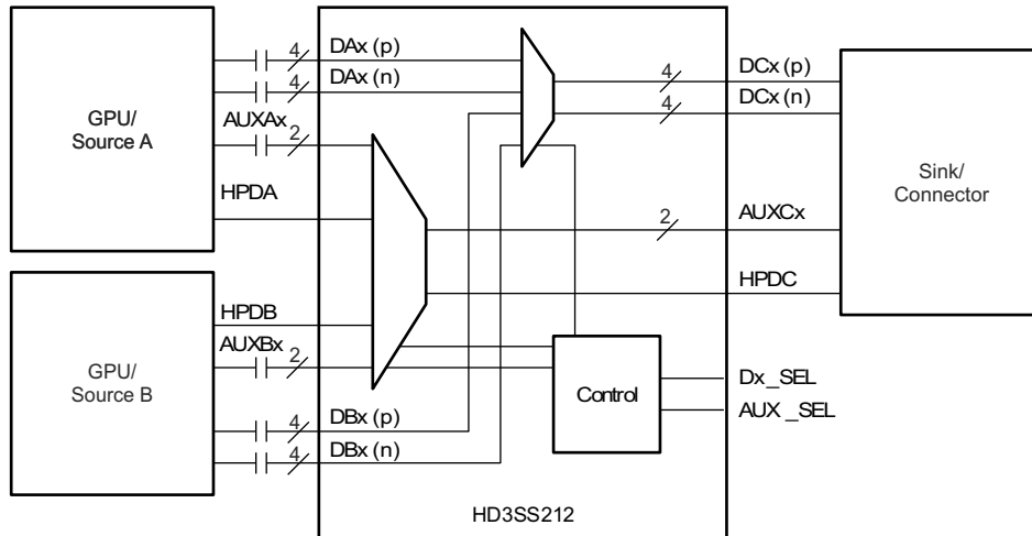
9-4. Dual Source Connection Block Diagram
