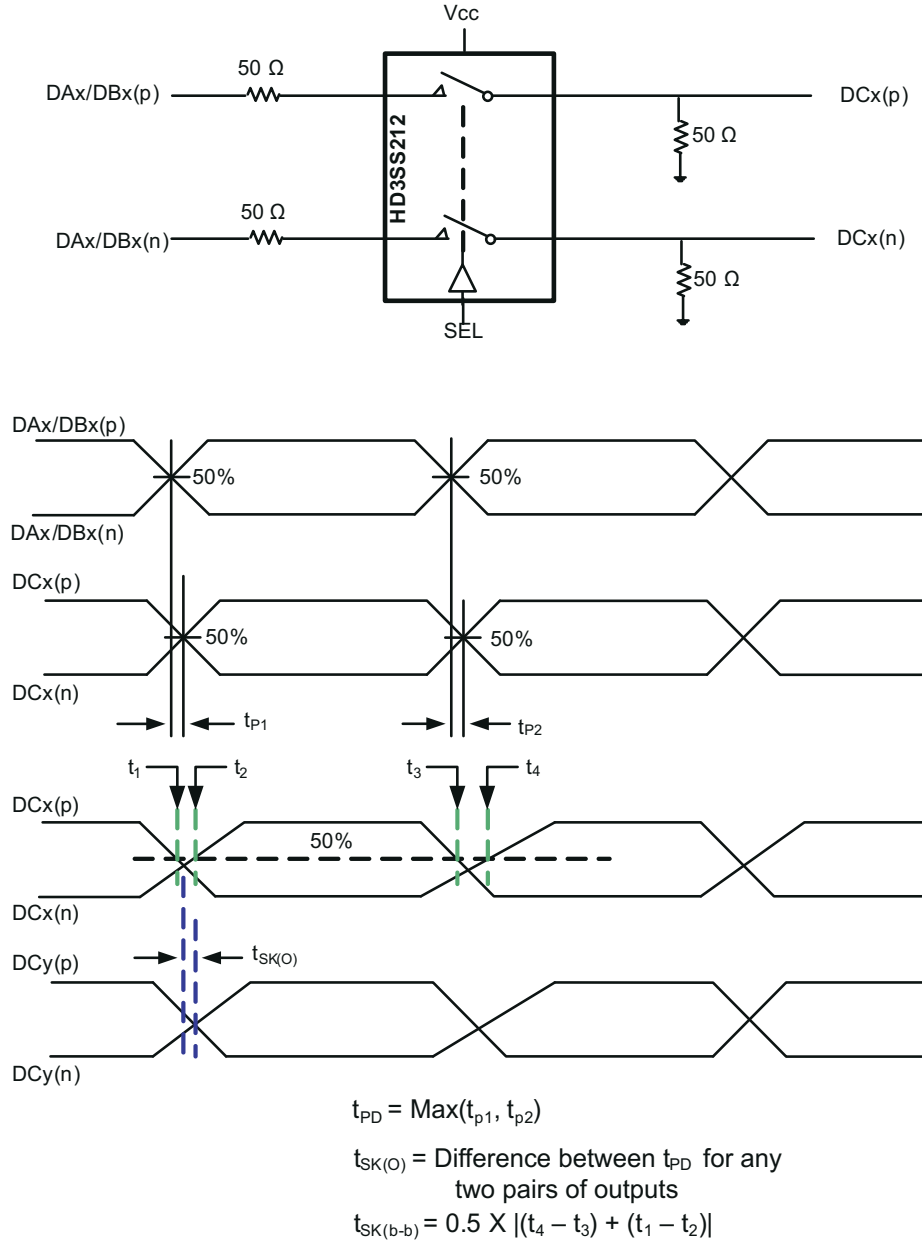
7-2. Propagation Delay and Skew
