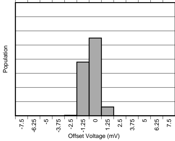
Fig 7. Bus Offset Voltage Production Distribution
