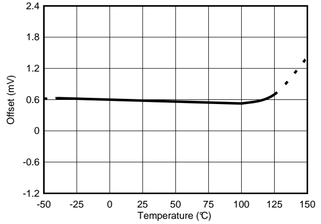
Fig 8. Bus Offset Voltage vs Temperature
