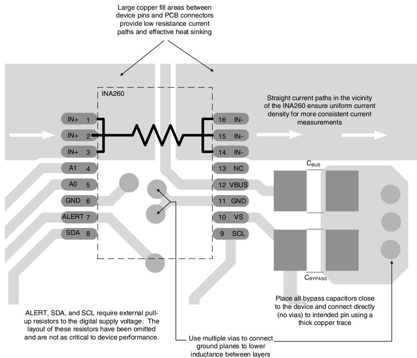
☒ 41. INA260 Layout Example
