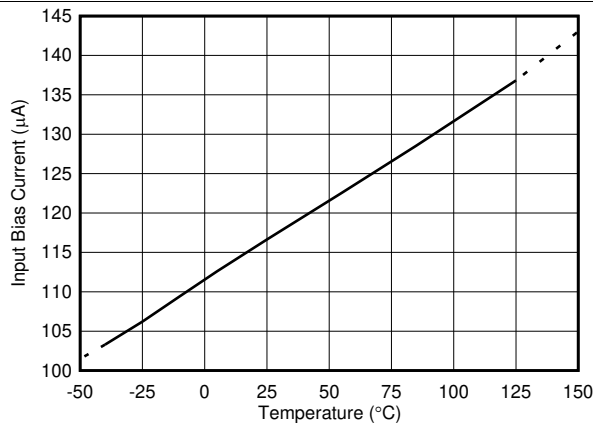
19. Input Bias Current vs Temperature
