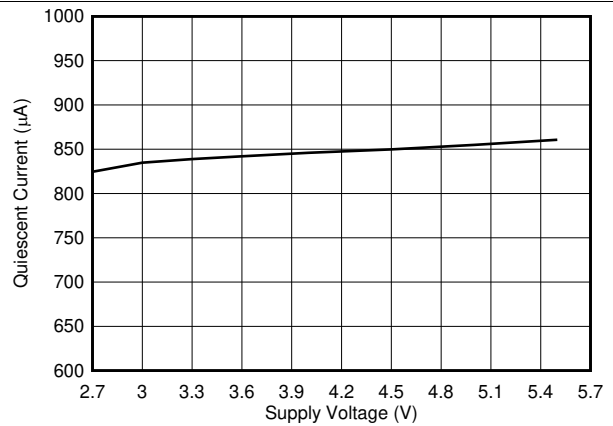
20. Quiescent Current vs Supply Voltage
