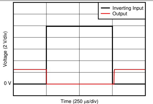
27. Step Response
