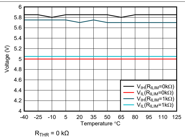
5-6. Input Voltage Threshold vs Temperature in Sink Mode
