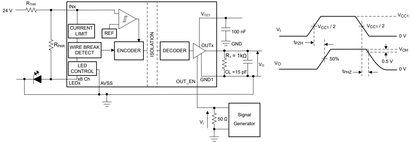
图 6-4. Enable and Disable Propagation Delay Time Test Circuit and Waveform—Logic High State
