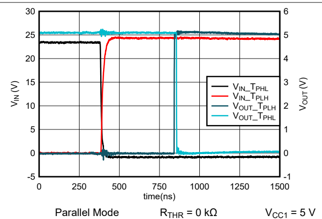
5-8. Propagation delay
