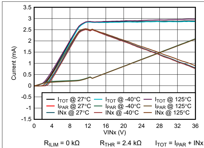
5-1. Input Current vs Input Voltage in Sink Mode
