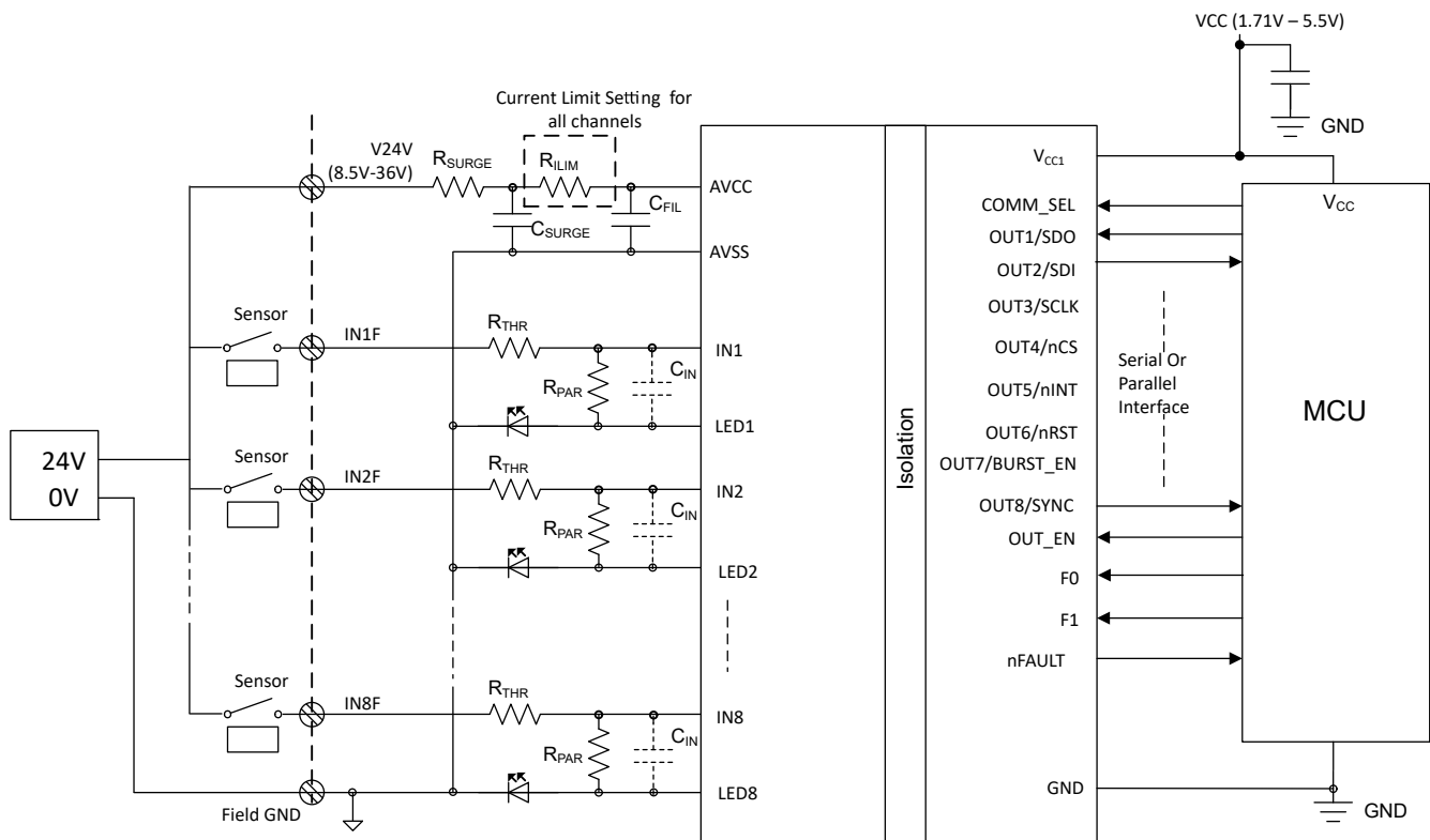
图 8-2. Sinking Type Digital Inputs with ISO1228
