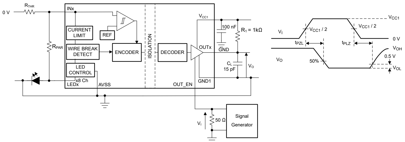
図 6-3. Enable and Disable Propagation Delay Time Test Circuit and Waveform—Logic Low State
