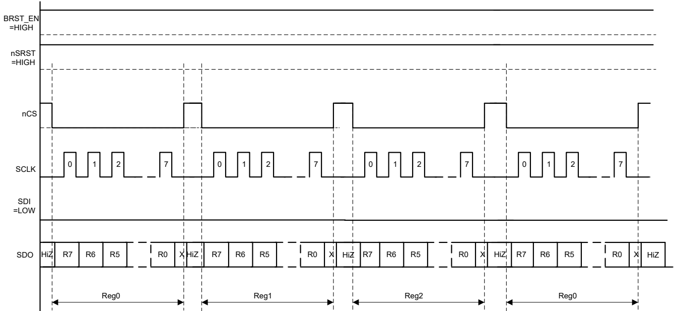
7-6. SPI Burst Mode Timing Block Diagram
