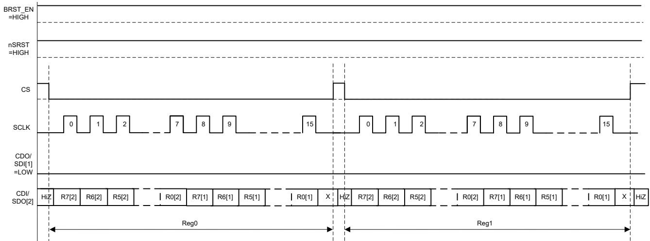
7-7. SPI Burst Mode Timing Diagram in Daisy Chain
