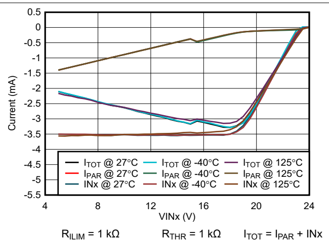
5-4. Input Current vs Input Voltage in Source Mode
