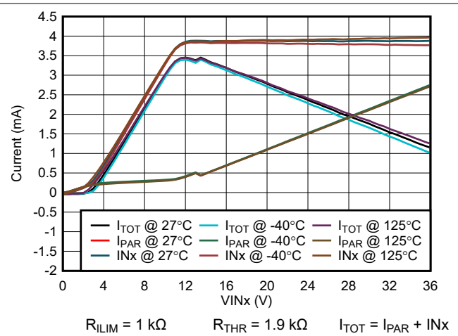
5-2. Input Current vs Input Voltage in Sink Mode
