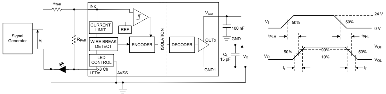
図 6-1. Switching Characteristics Test Circuit and Voltage Waveforms
