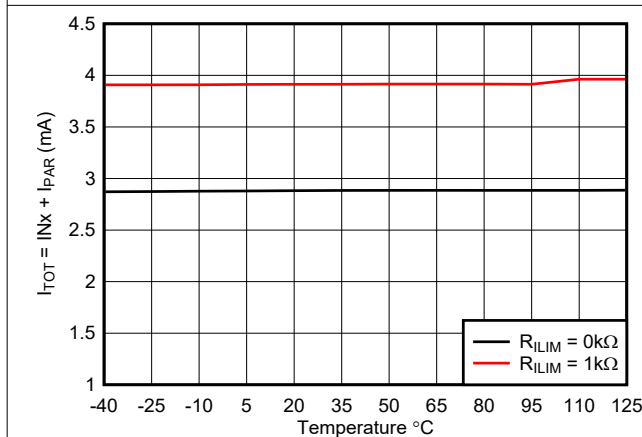
5-5. Input Current vs Temperature in Sink Mode
