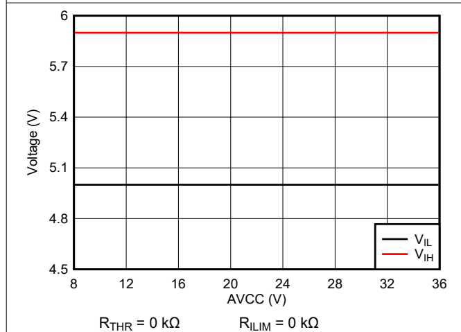
5-9. Input Voltage Threshold vs AVCC in Sink Mode
