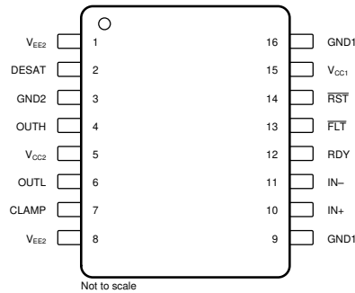
图 6-1. DWV Package 16-Pin SOIC Top View
