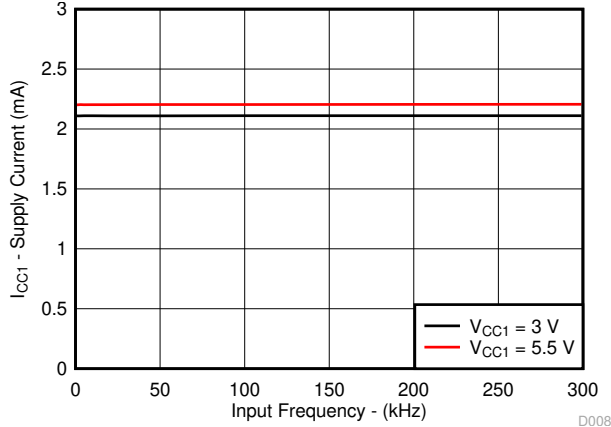
7-21. I_{CC1} Supply Current vs Input Frequency
