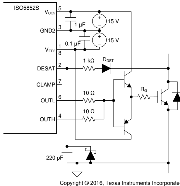
10-10. Current Buffer for Increased Drive Current
