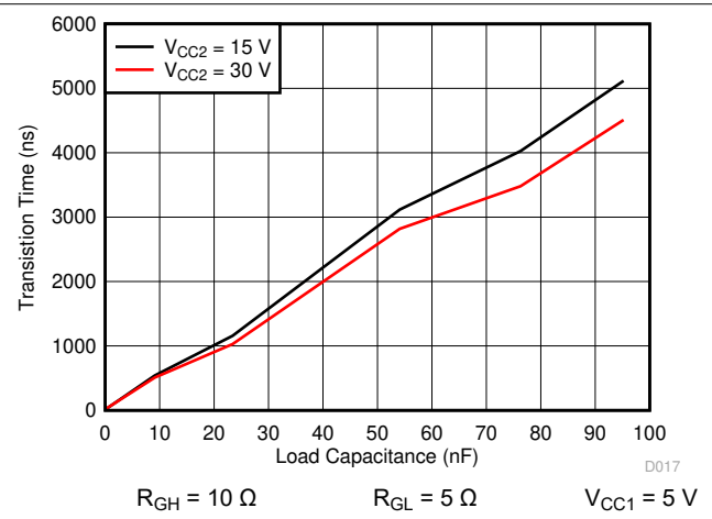
7-30. t_r Rise Time vs Load Capacitance
