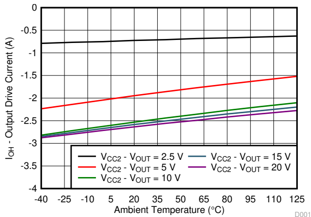
7-4. Output High Drive Current vs Temperature
