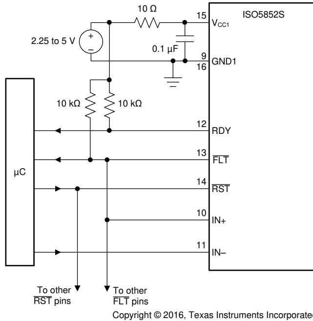
10-6. Global Shutdown With Inverting Input Configuration
