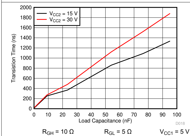
7-31. t_f Fall Time vs Load Capacitance
