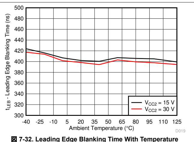
7-32. Leading Edge Blanking Time With Temperature
