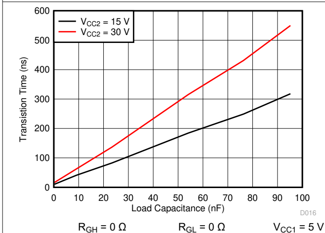
7-29. t_f Fall Time vs Load Capacitance
