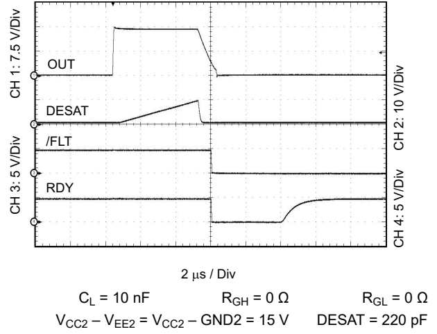
7-16. Output Transient Waveform DESAT, RDY, and \overline{\text{FLT}}
