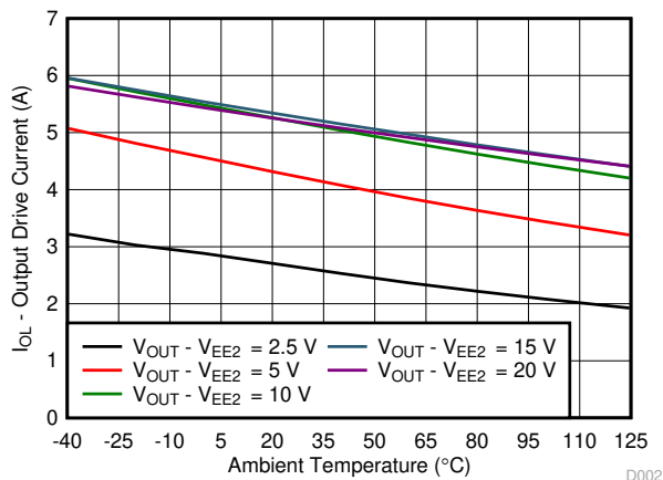
7-6. Output Low Drive Current vs Temperature
