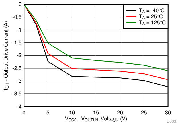
7-5. Output High Drive Current vs Output Voltage
