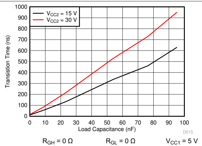
7-28. t_r Rise Time vs Load Capacitance
