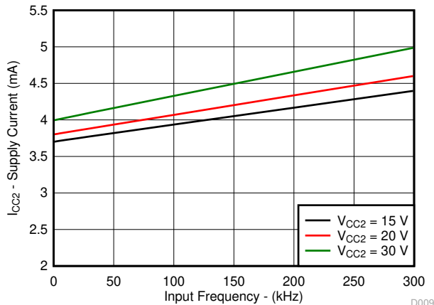
7-23. I_{CC2} Supply Current vs Input Frequency
