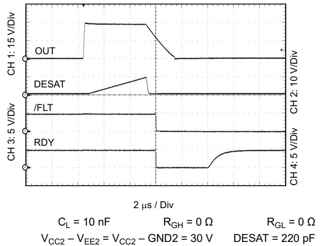
7-18. Output Transient Waveform DESAT, RDY, and \overline{\text{FLT}}
