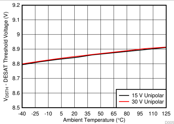
7-8. DESAT Threshold Voltage vs Temperature Unipolar: V_{CC2} - V_{EE2} = V_{CC2} - GND2
